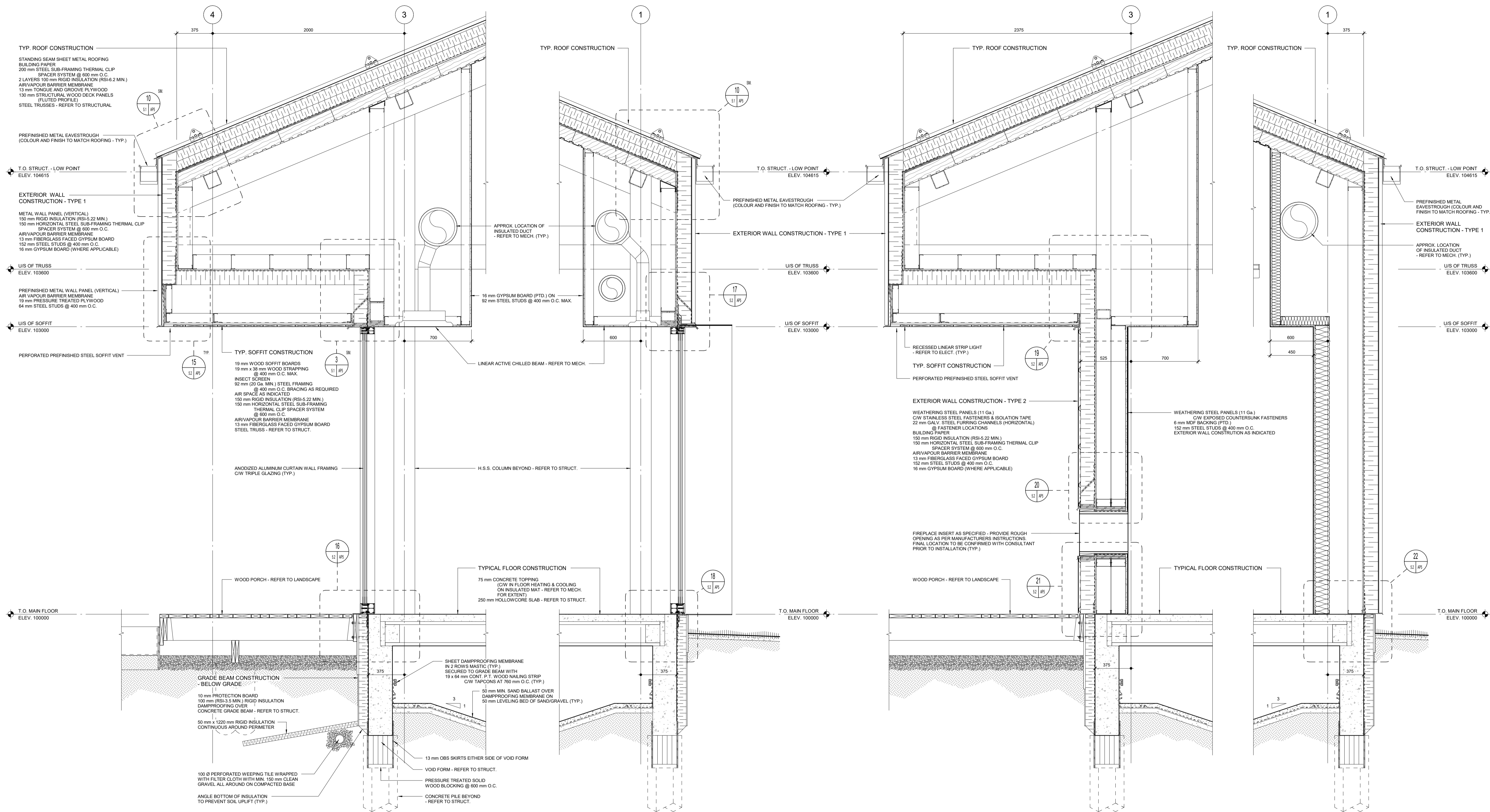
4 TYP. SECTION THRU OPEN LIBRARY GLAZING SCALE 1:20
