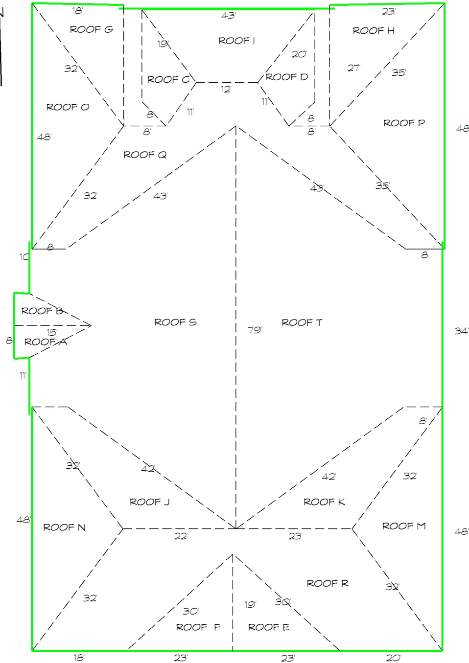
BUILDING ROOF PLAN
