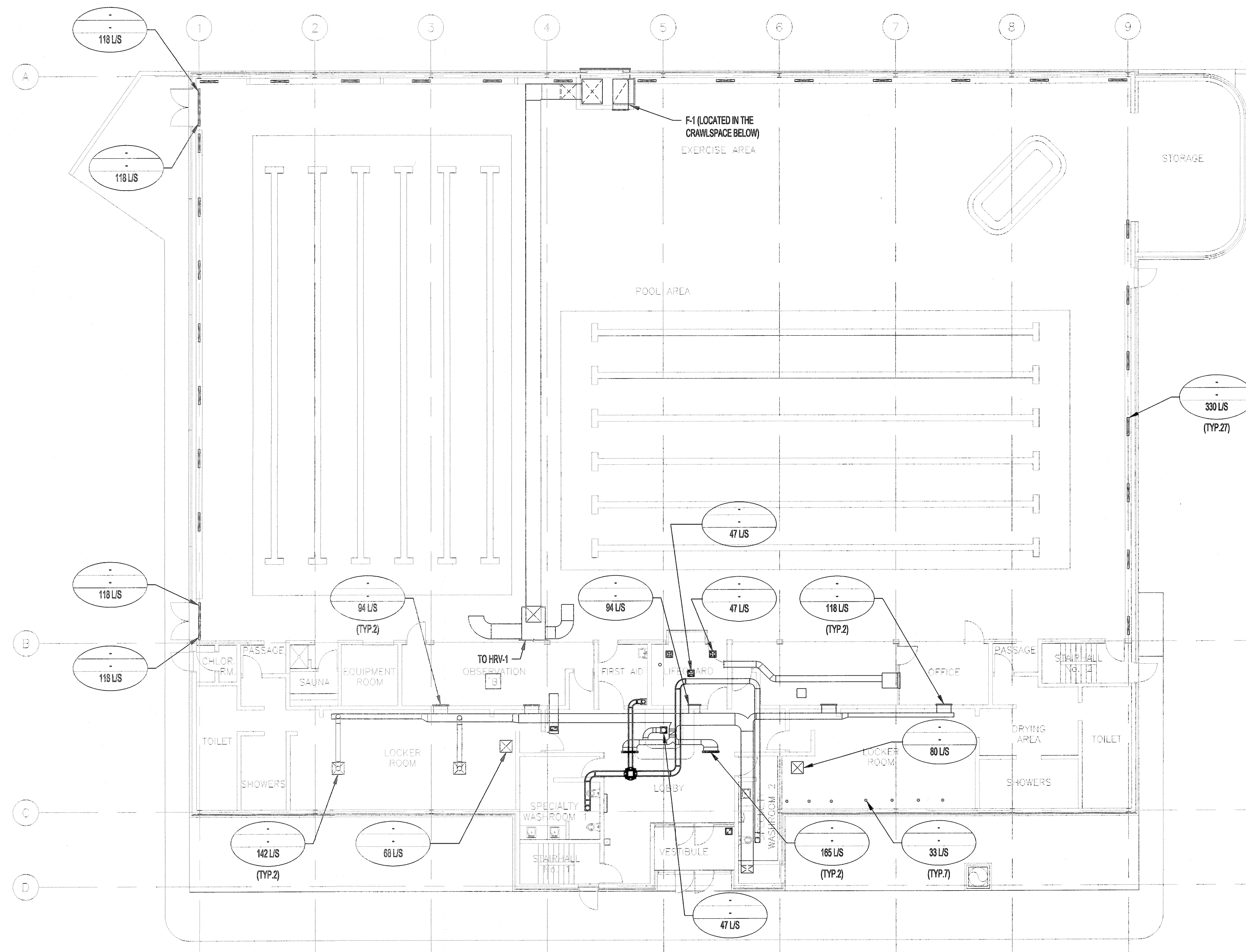
MAIN FLOOR PLAN SCALE 1:150
