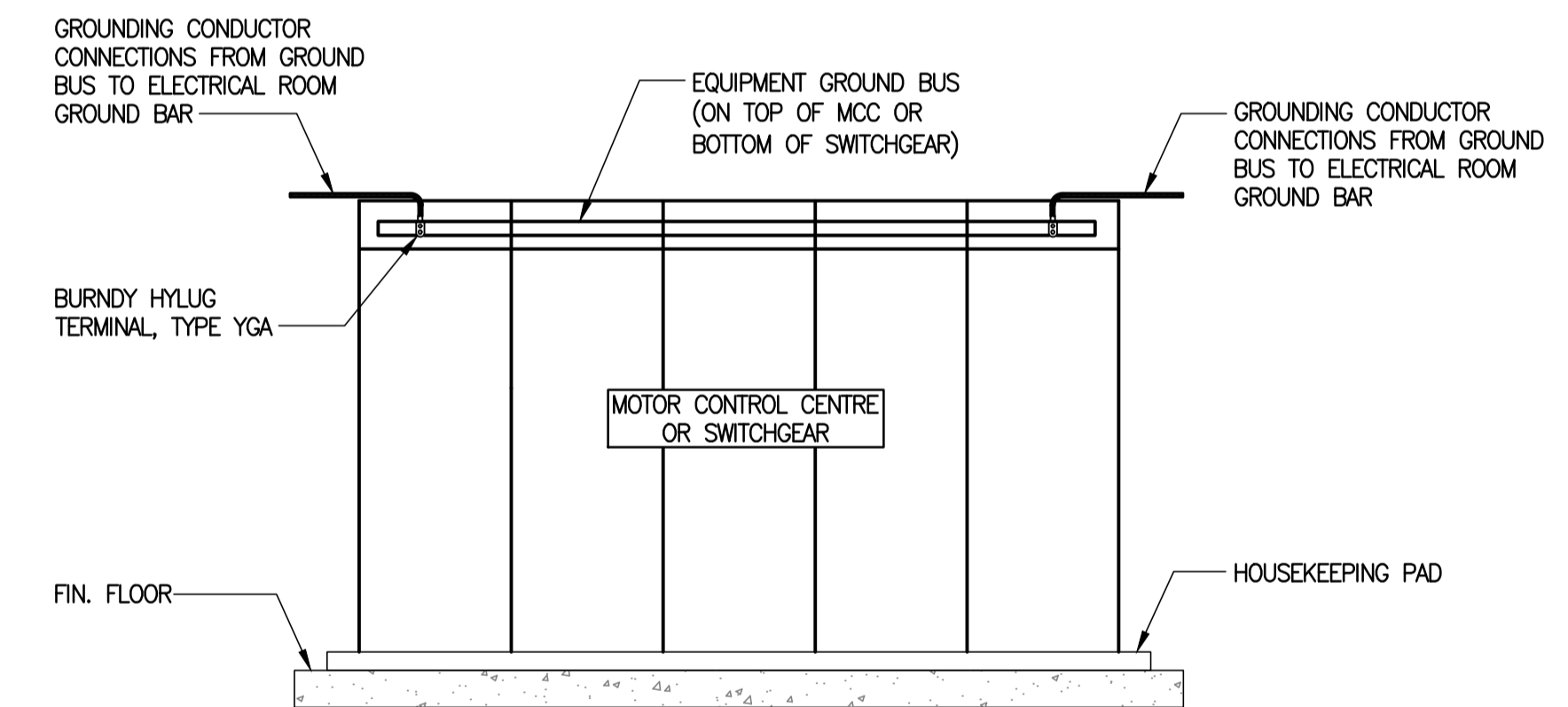
2 MCC OR SWITCHGEAR GROUNDING CONNECTIONS SCALE: N.T.S.
