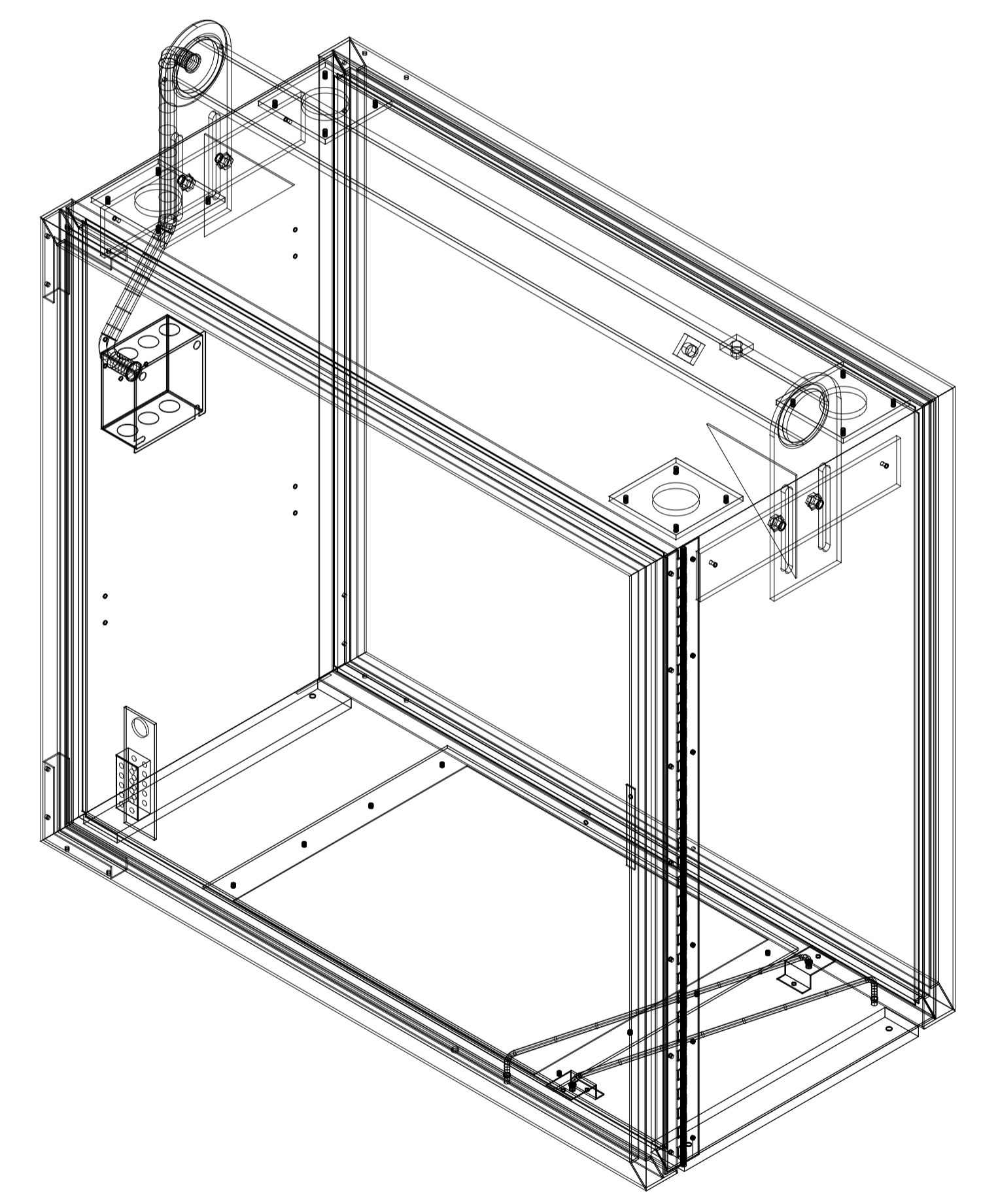
ISOMETRIC VIEW
