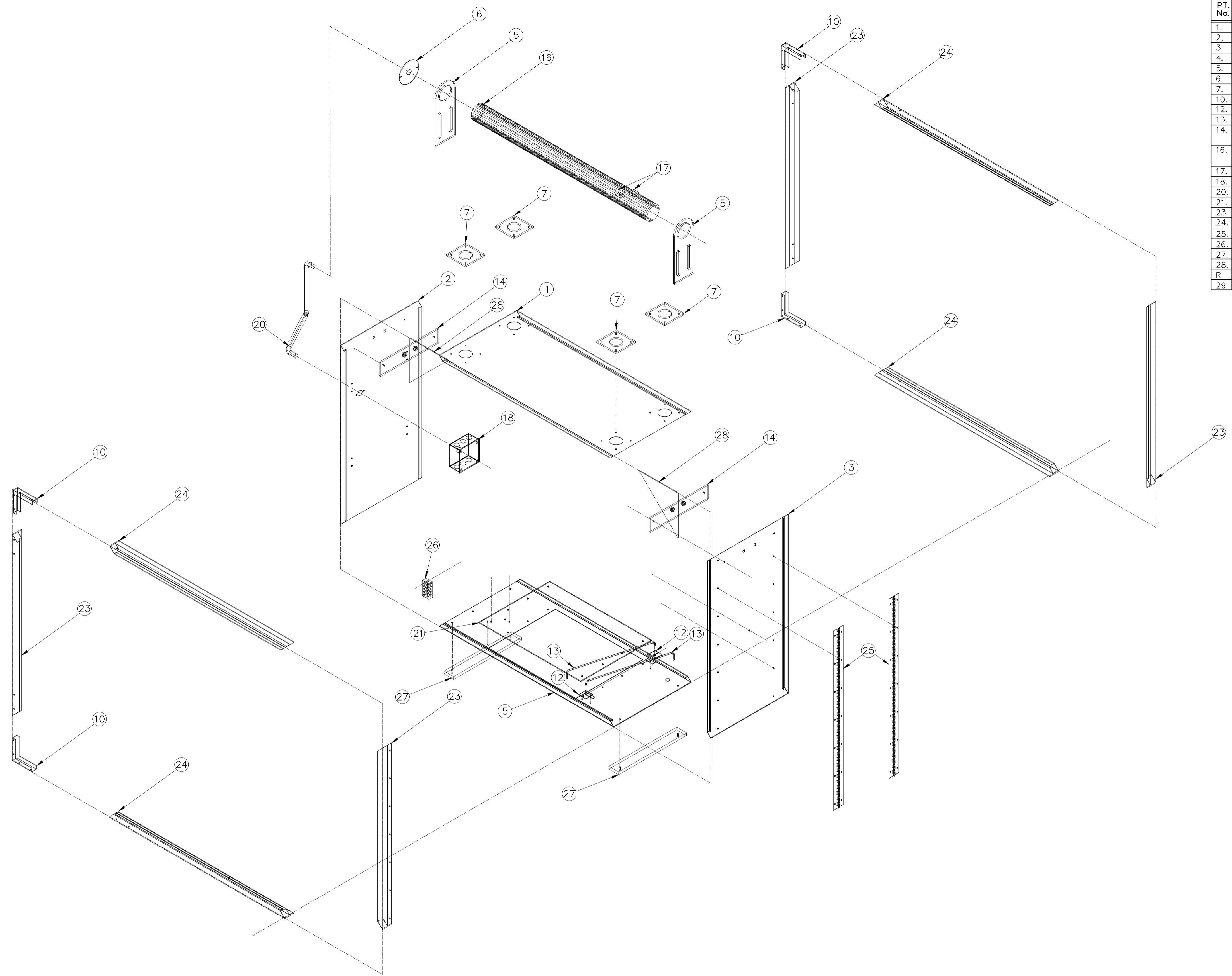
ASSEMBLY VIEW
