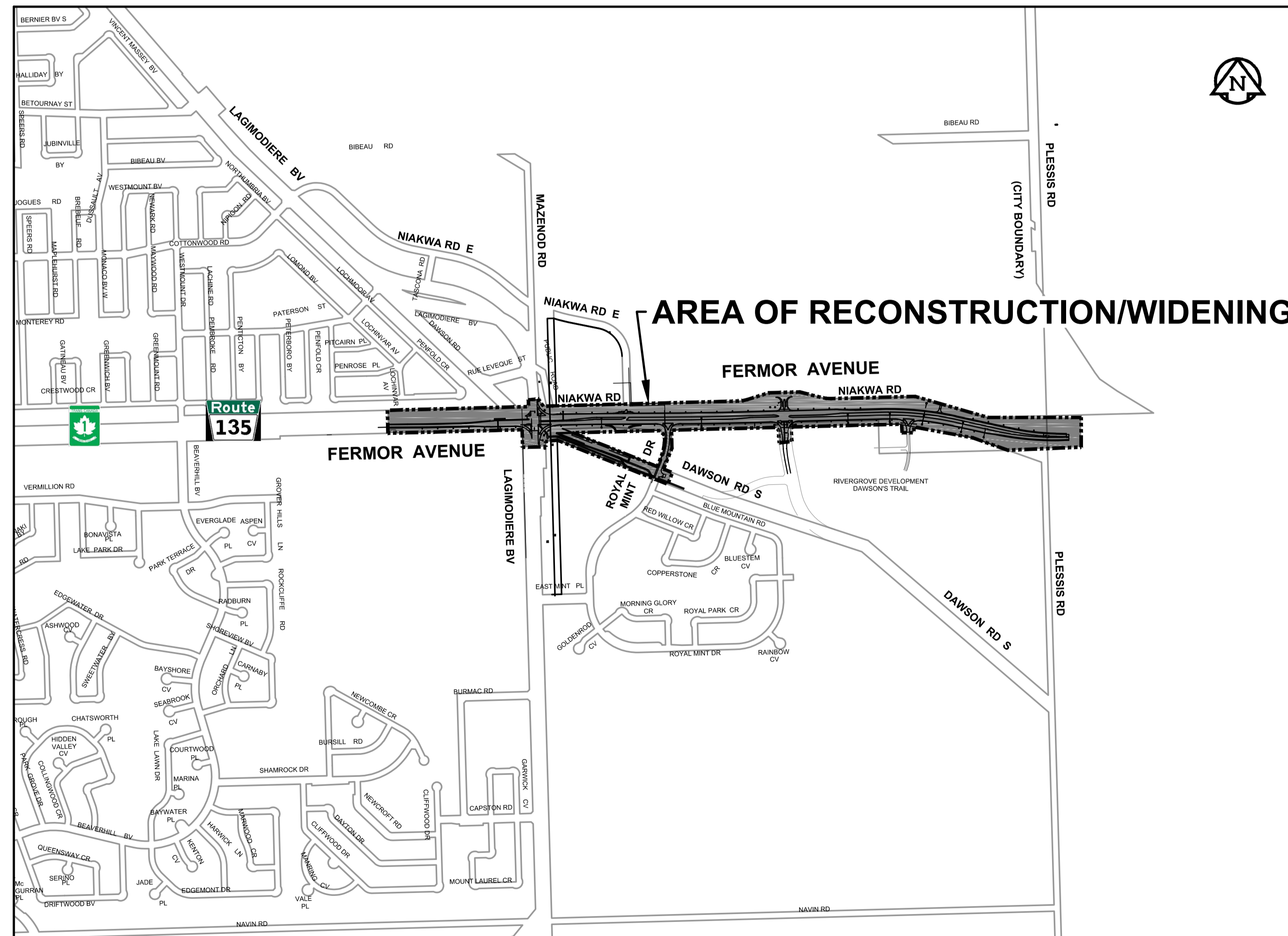
LOCATION PLAN SCALE: 1:10,000 0 250 500m
