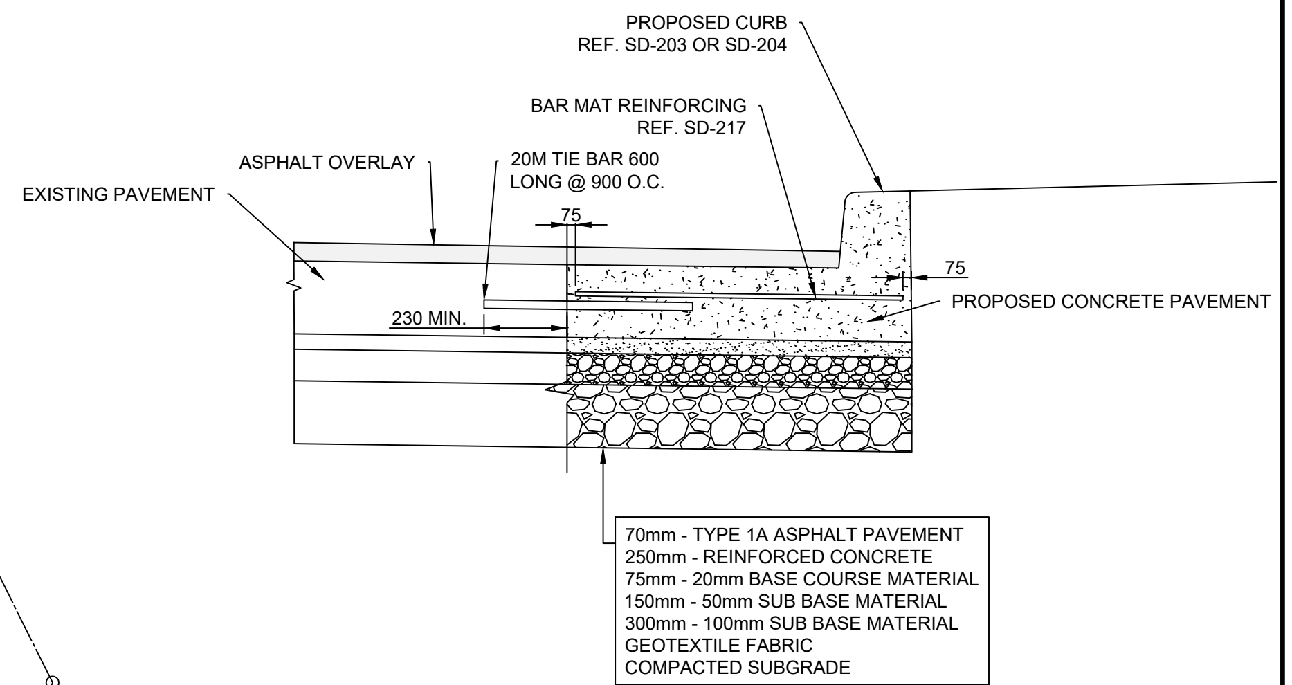
ST VITAL PARK APPROACH - PAVEMENT WIDENING N.T.S.
