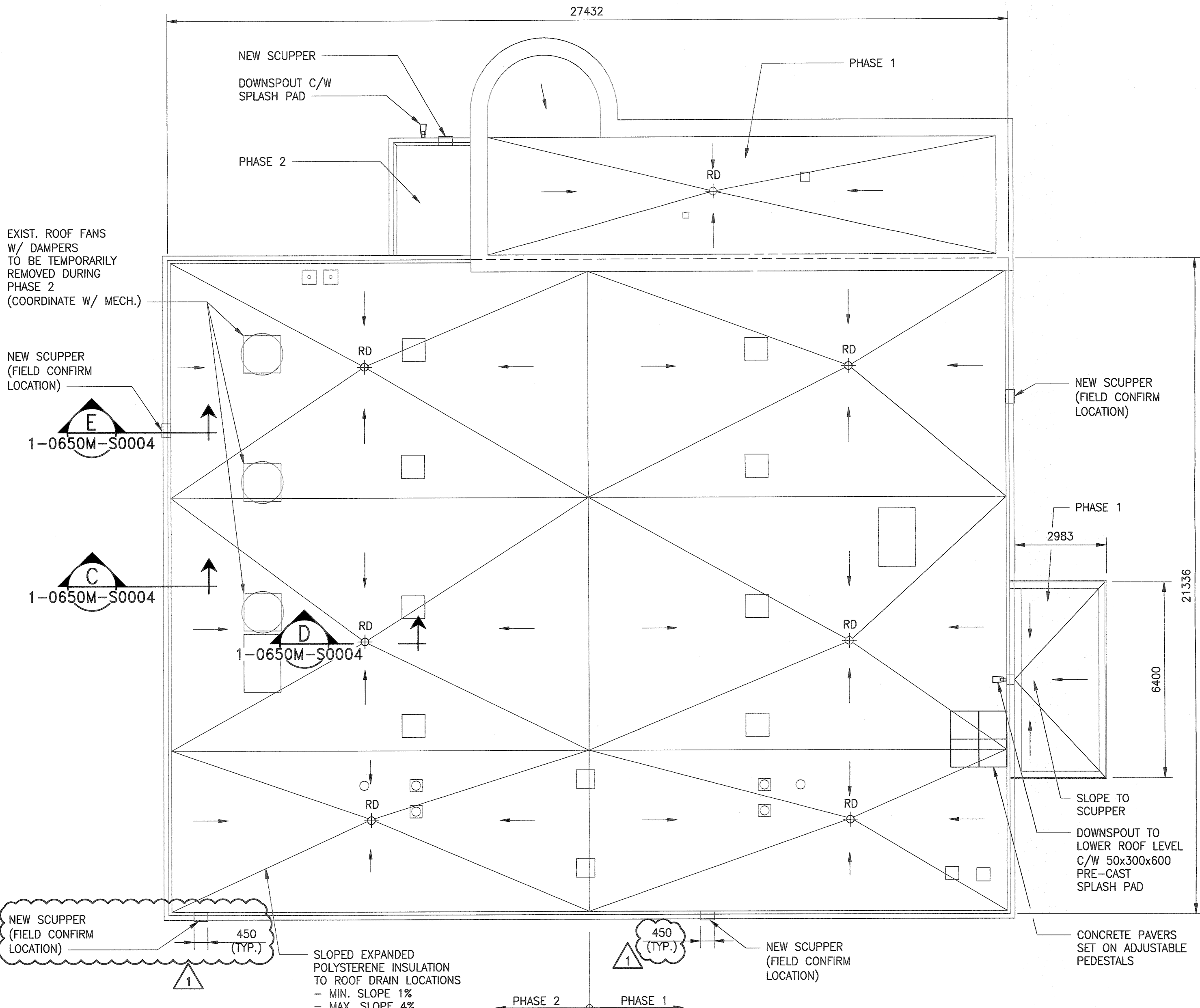
ROOF PLAN SCALE: 1:100
