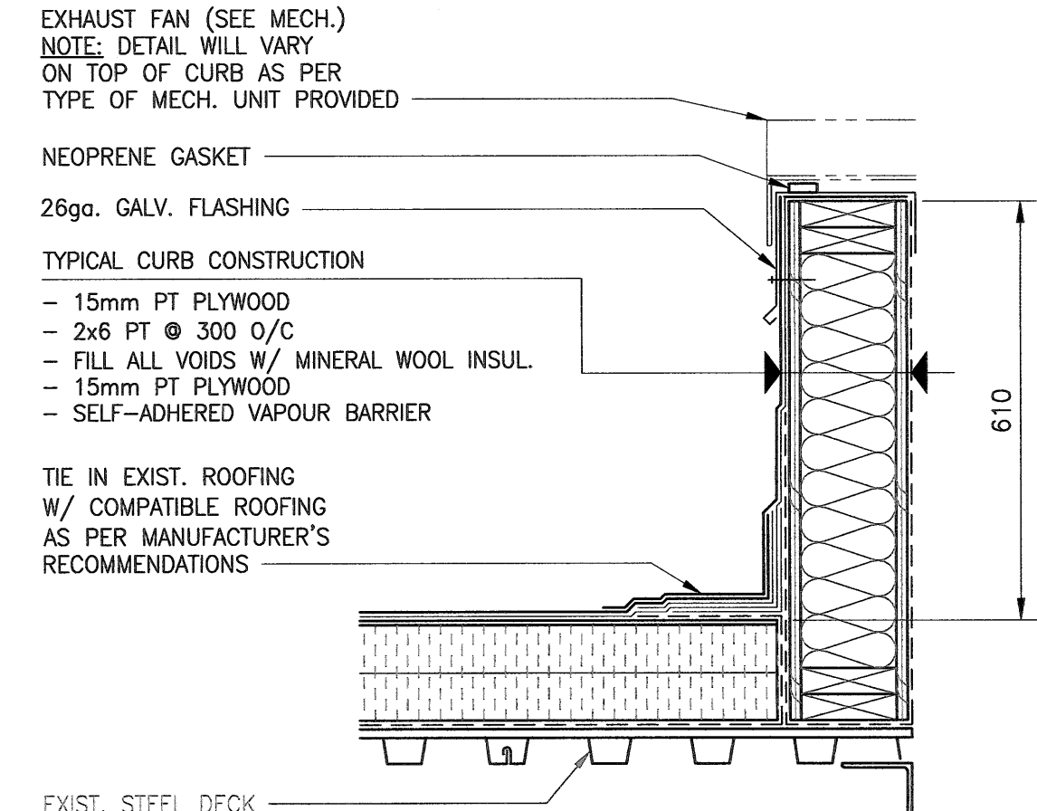
DETAIL - TYPICAL FAN CURB SCALE: 1:10
