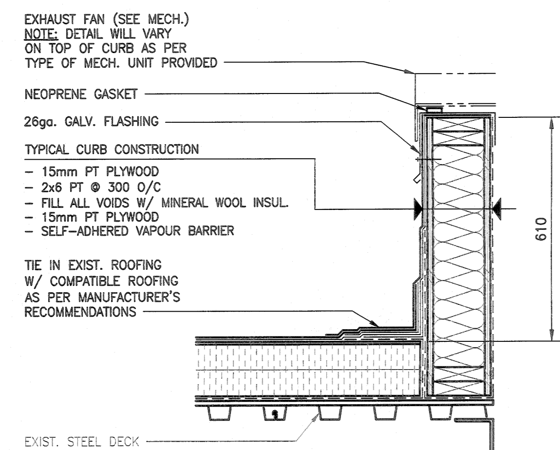
DETAIL - TYPICAL FAN CURB SCALE: 1:10
