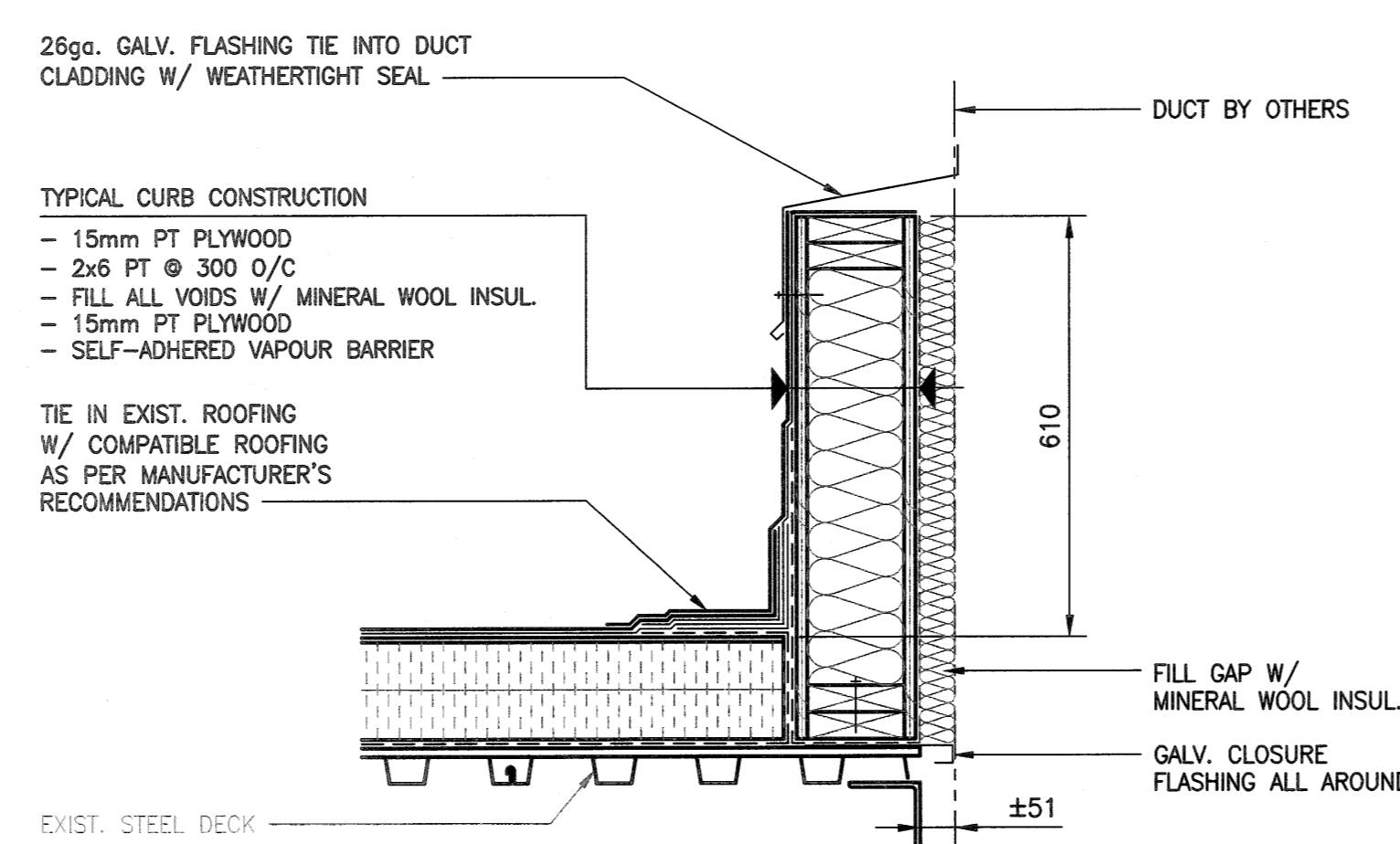
DETAIL - TYPICAL DUCT PENETRATION SCALE: 1:10
