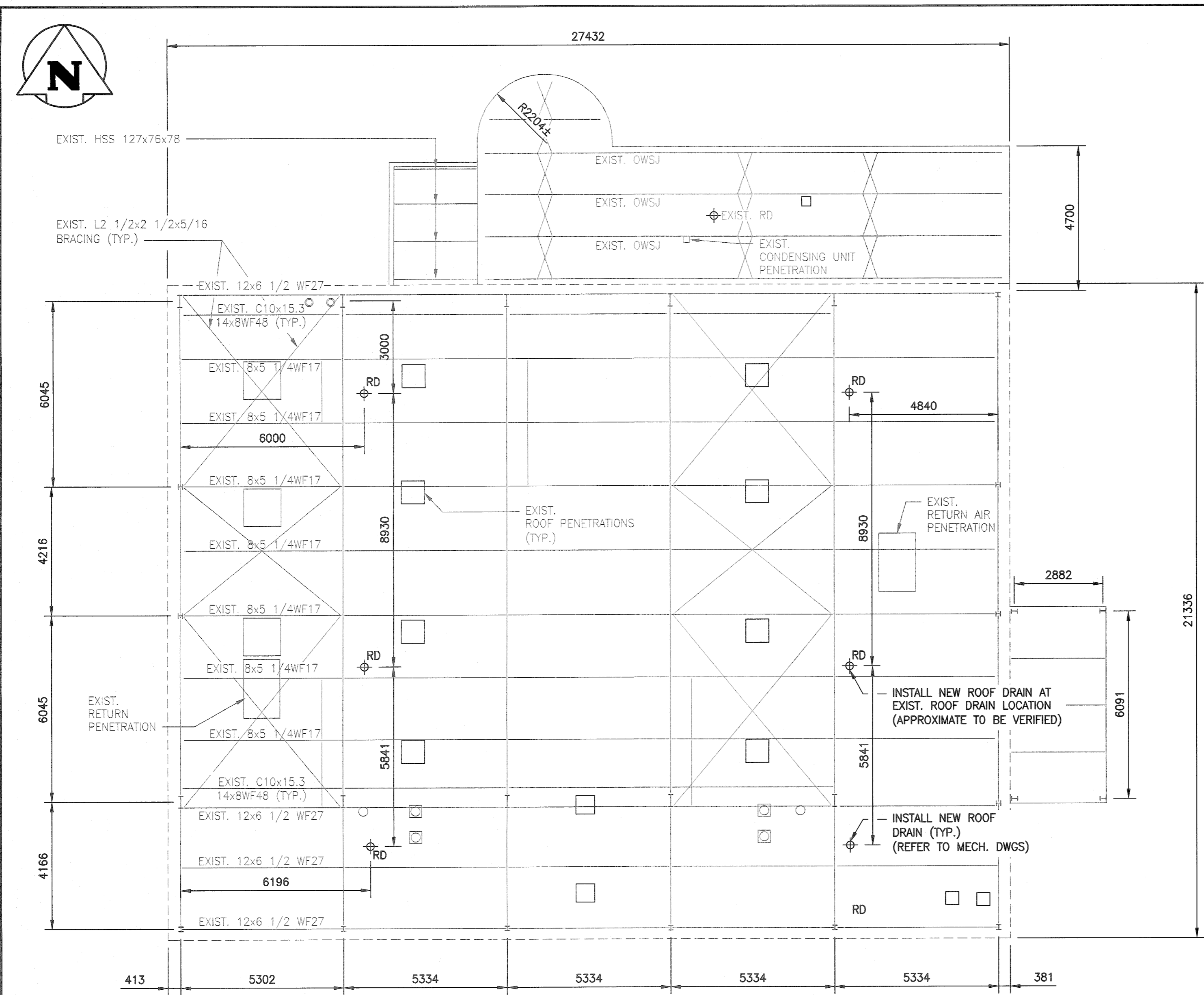
ROOF FRAMING PLAN SCALE: 1:100
