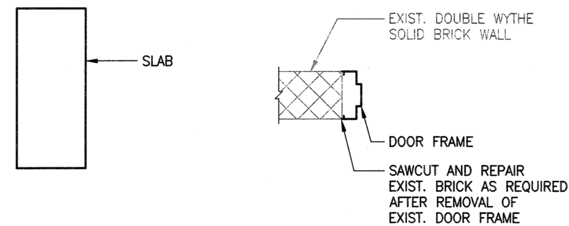
DETAIL - DOOR/JAMB
