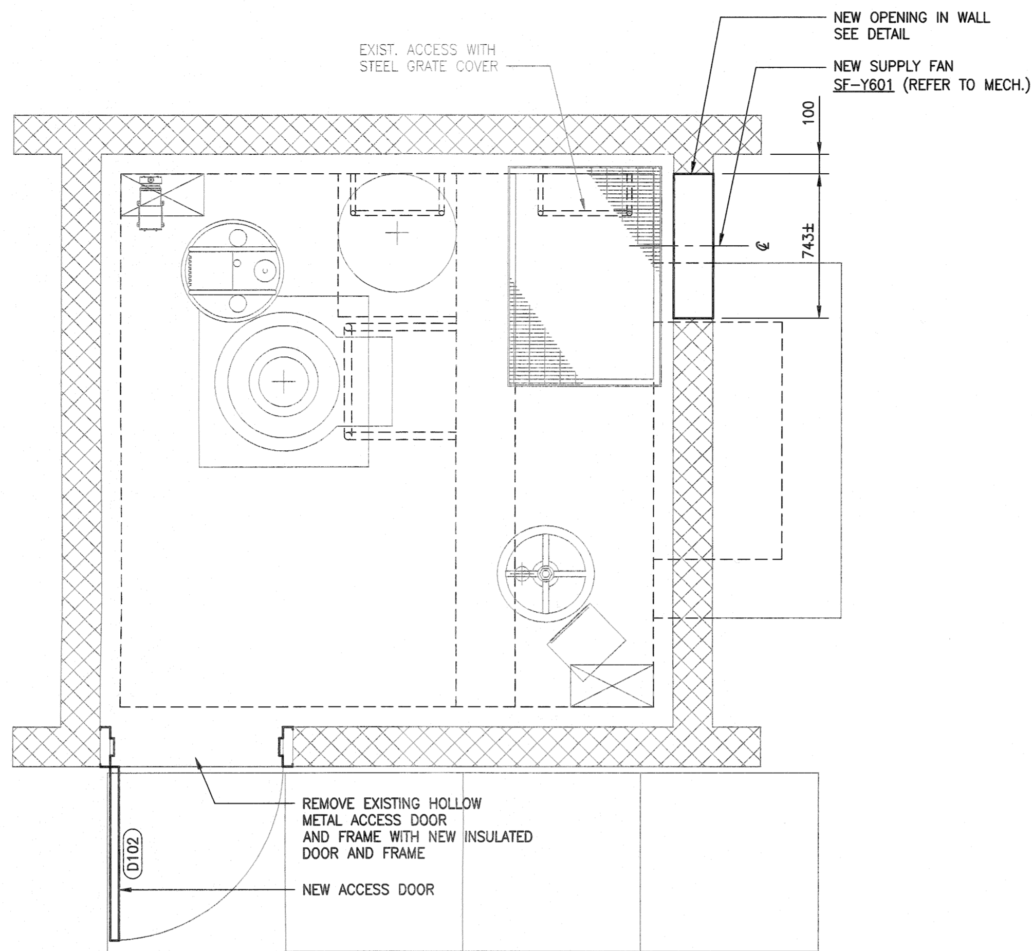
PLAN VIEW - HURST DRAINAGE LIFT STATION
