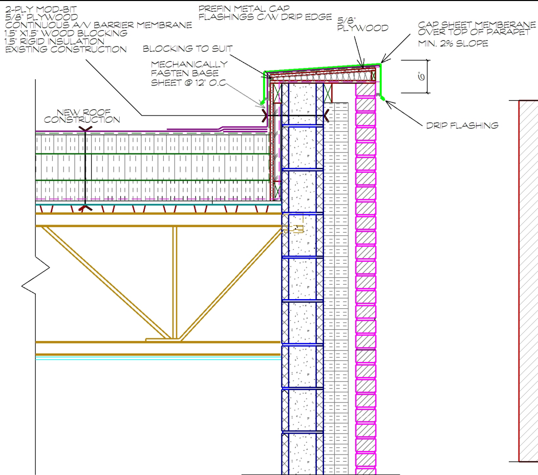
PARAPET DETAILS
