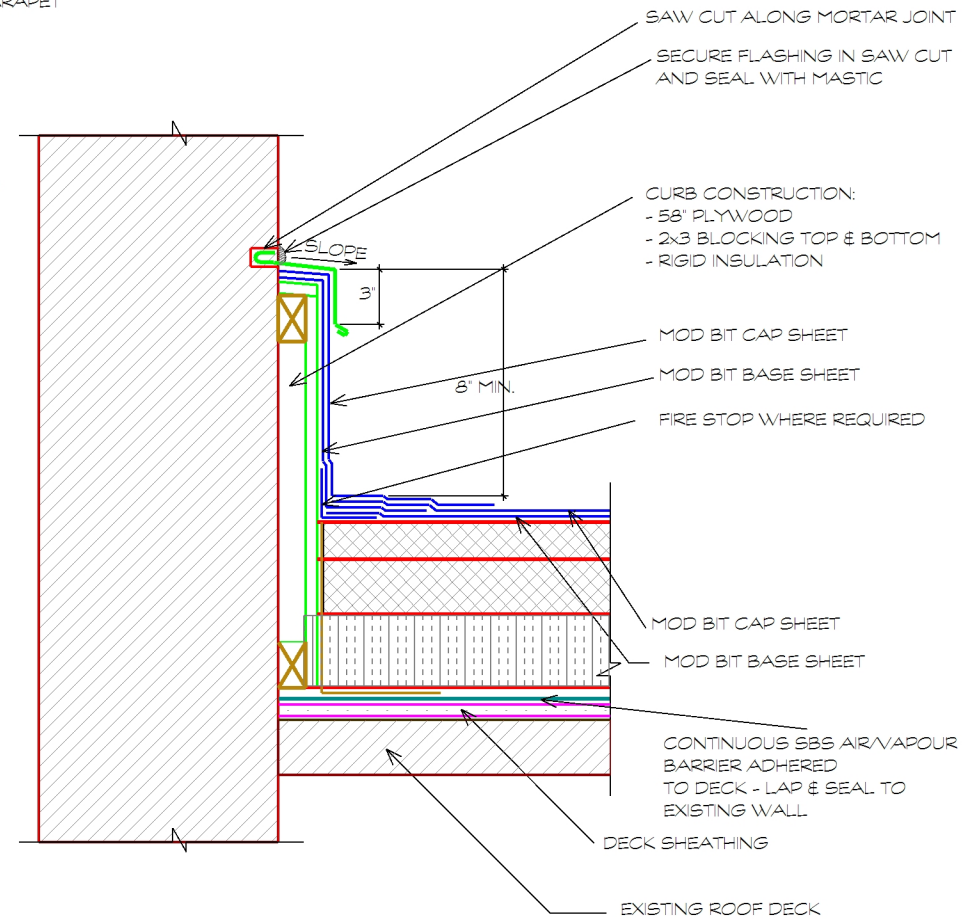
TYPICAL MASONRY DETAIL
