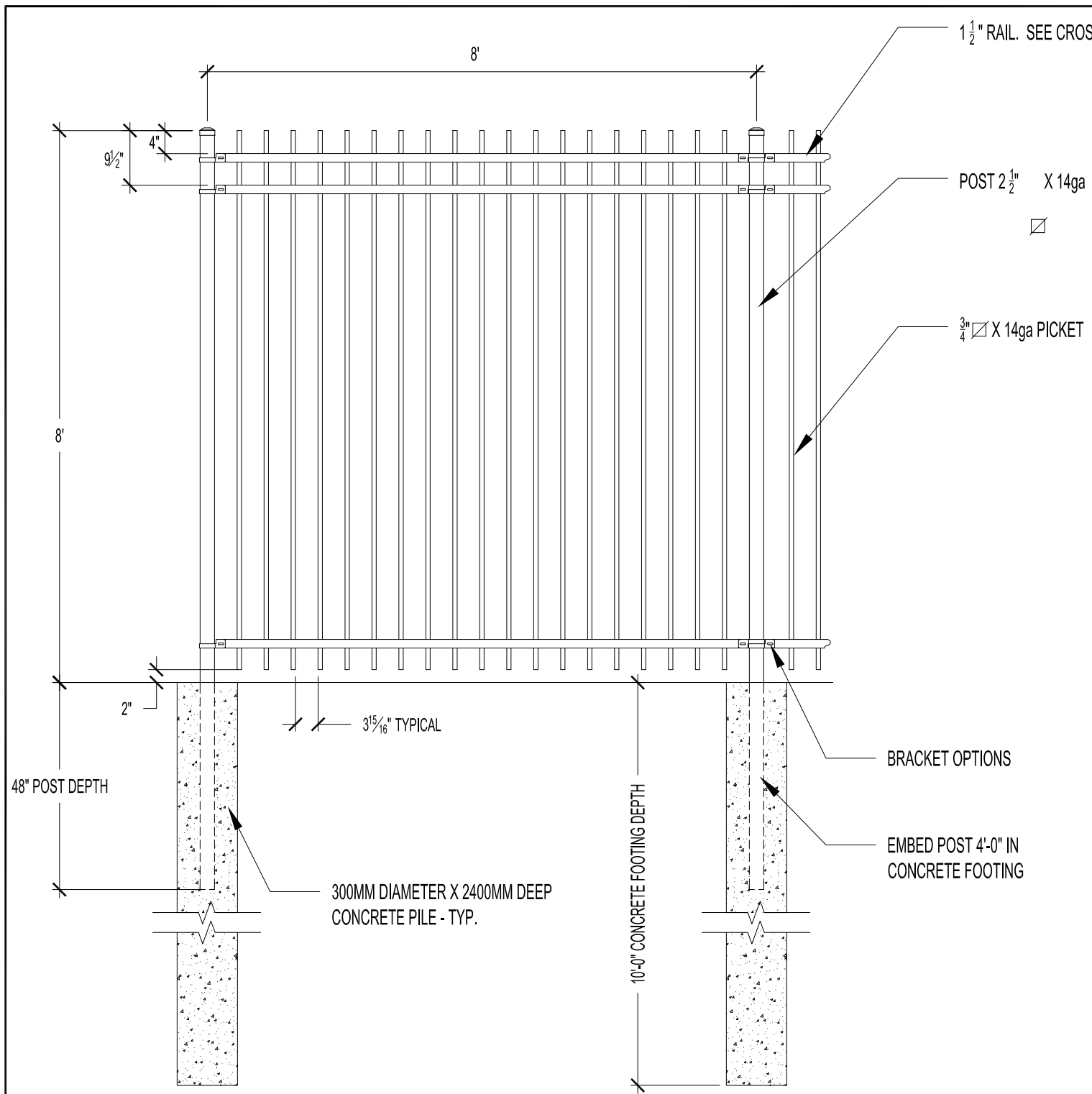
1 FENCE DETAIL SCALE 1/2" = 1'-0"
