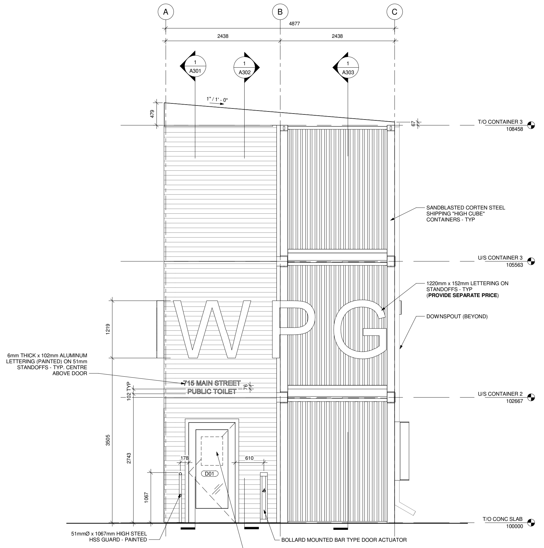
1 EXTERIOR ELEVATION - WEST 1 : 48
