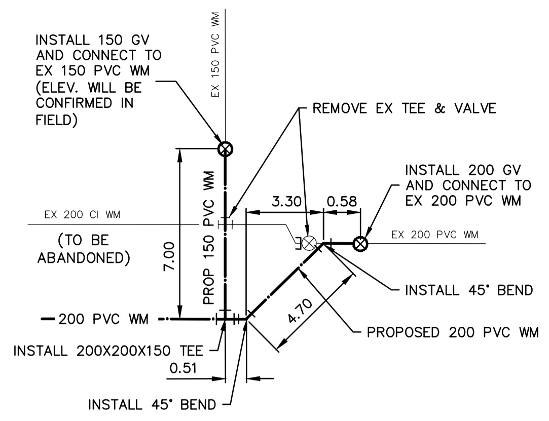
DETAIL "A" CONNECTION AT BISSETT CR SCALE N.T.S.
