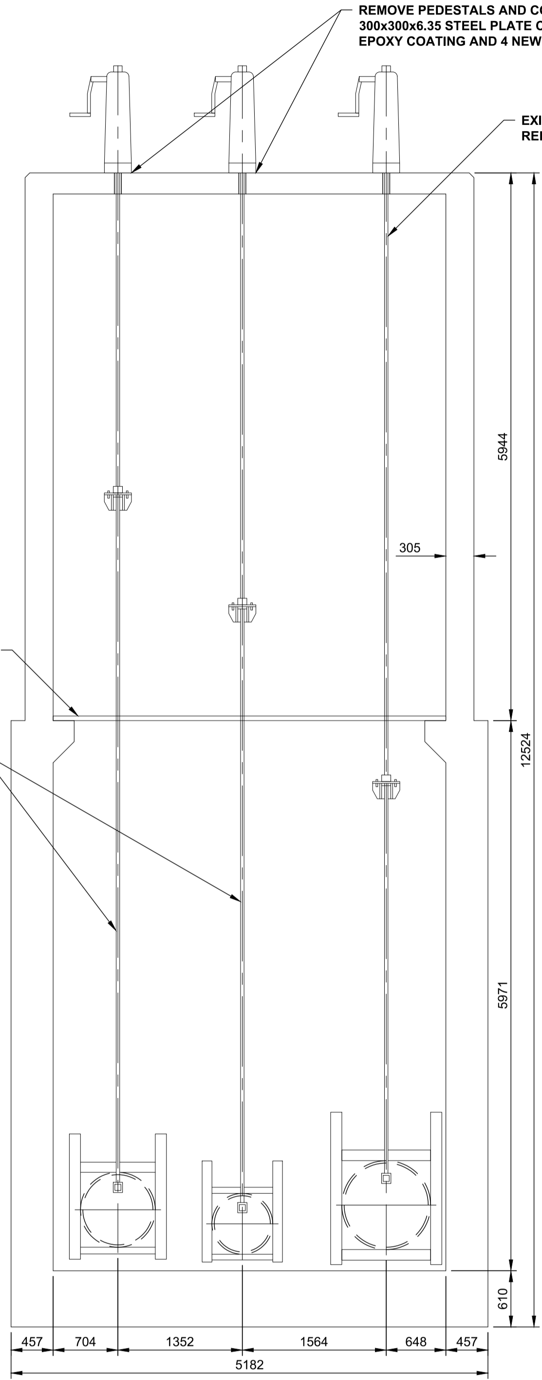
B SECTION
