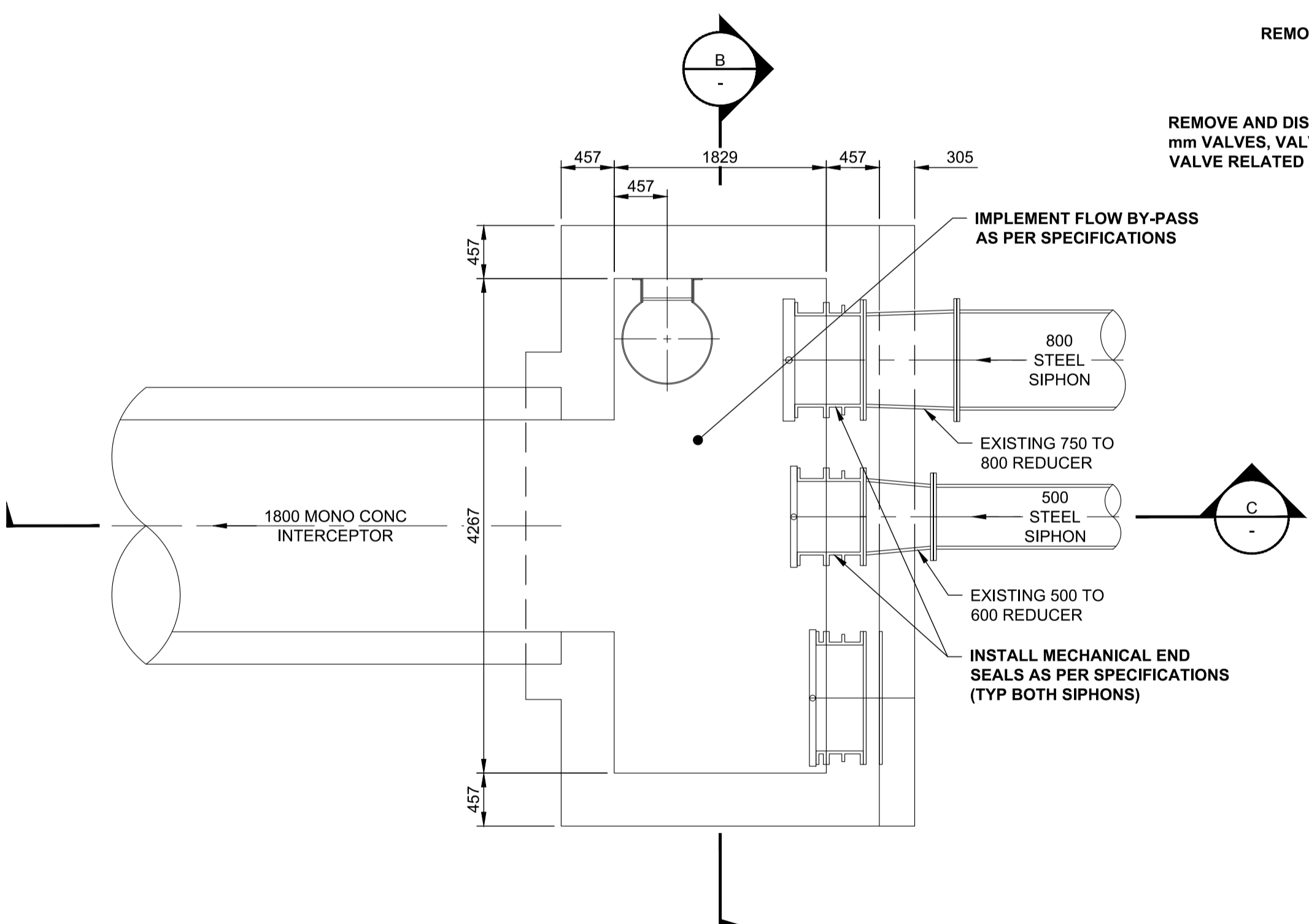
A SECTION FLOOR PLAN
