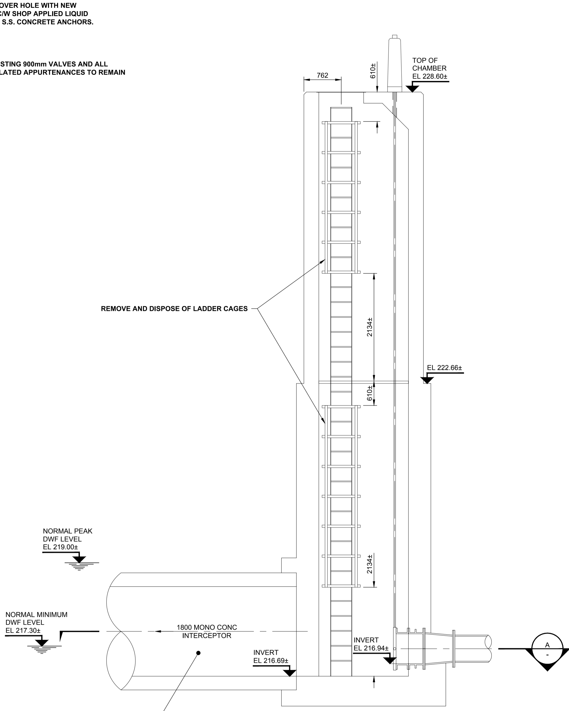
C SECTION
