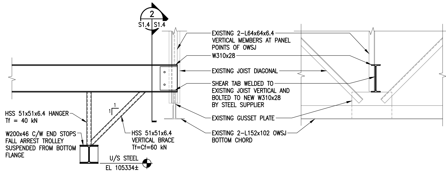
1 SECTION S1.2 | S1.4 1:20
