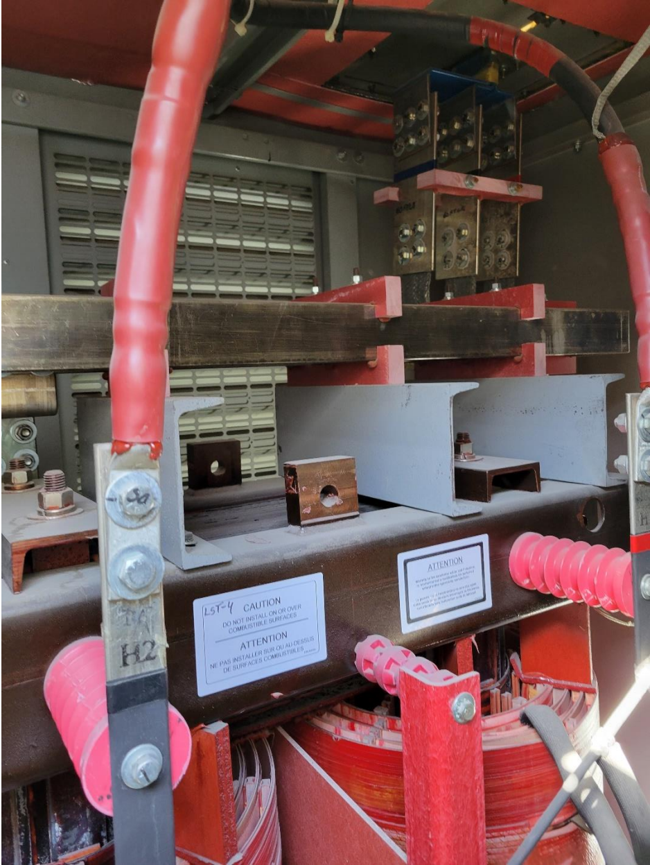
Transformer LST-4 Photo 3
