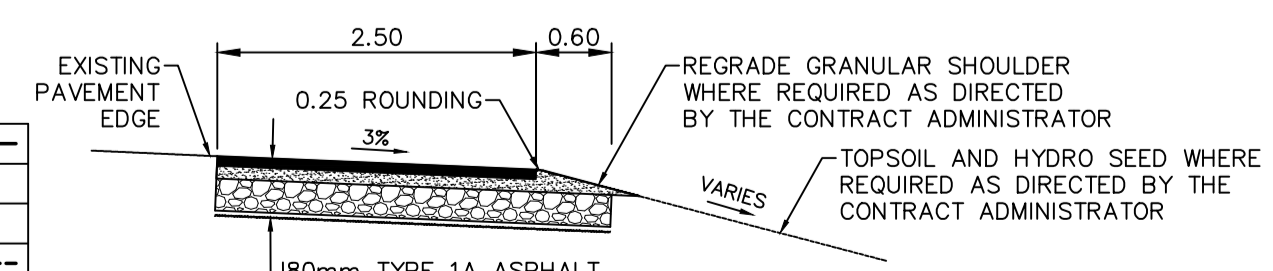
TYPICAL CROSS-SECTION NTS
