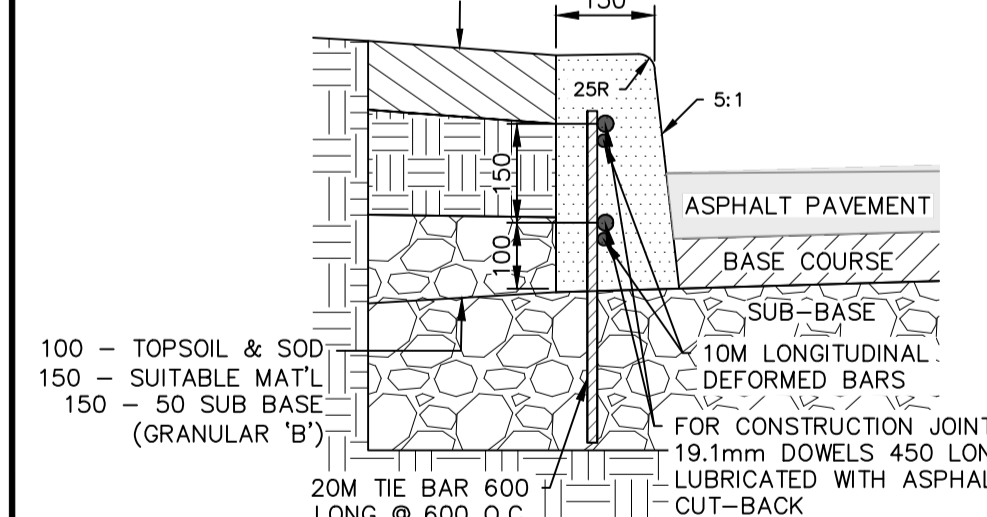
DETAIL 'A' - DOWELLED BARRIER CURB (SD-200A)
