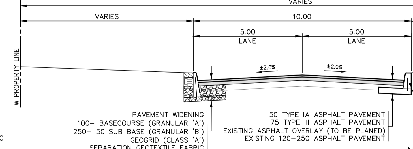
TYPICAL CROSS-SECTION SCALE 1:100
