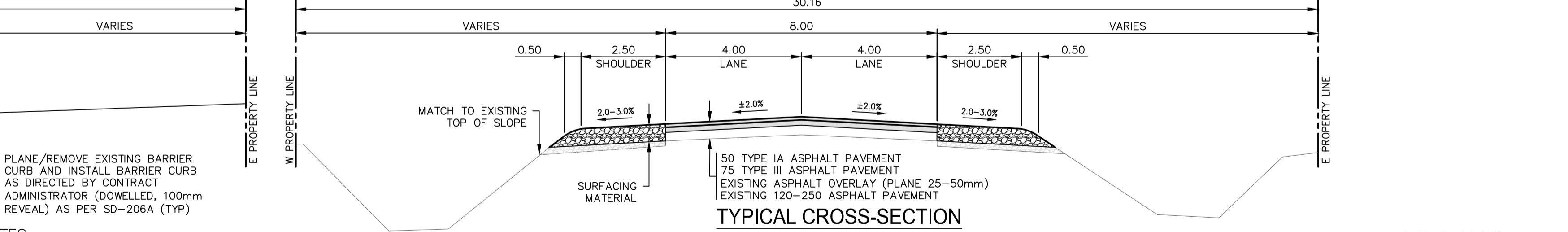
TYPICAL CROSS-SECTION SCALE 1:100
