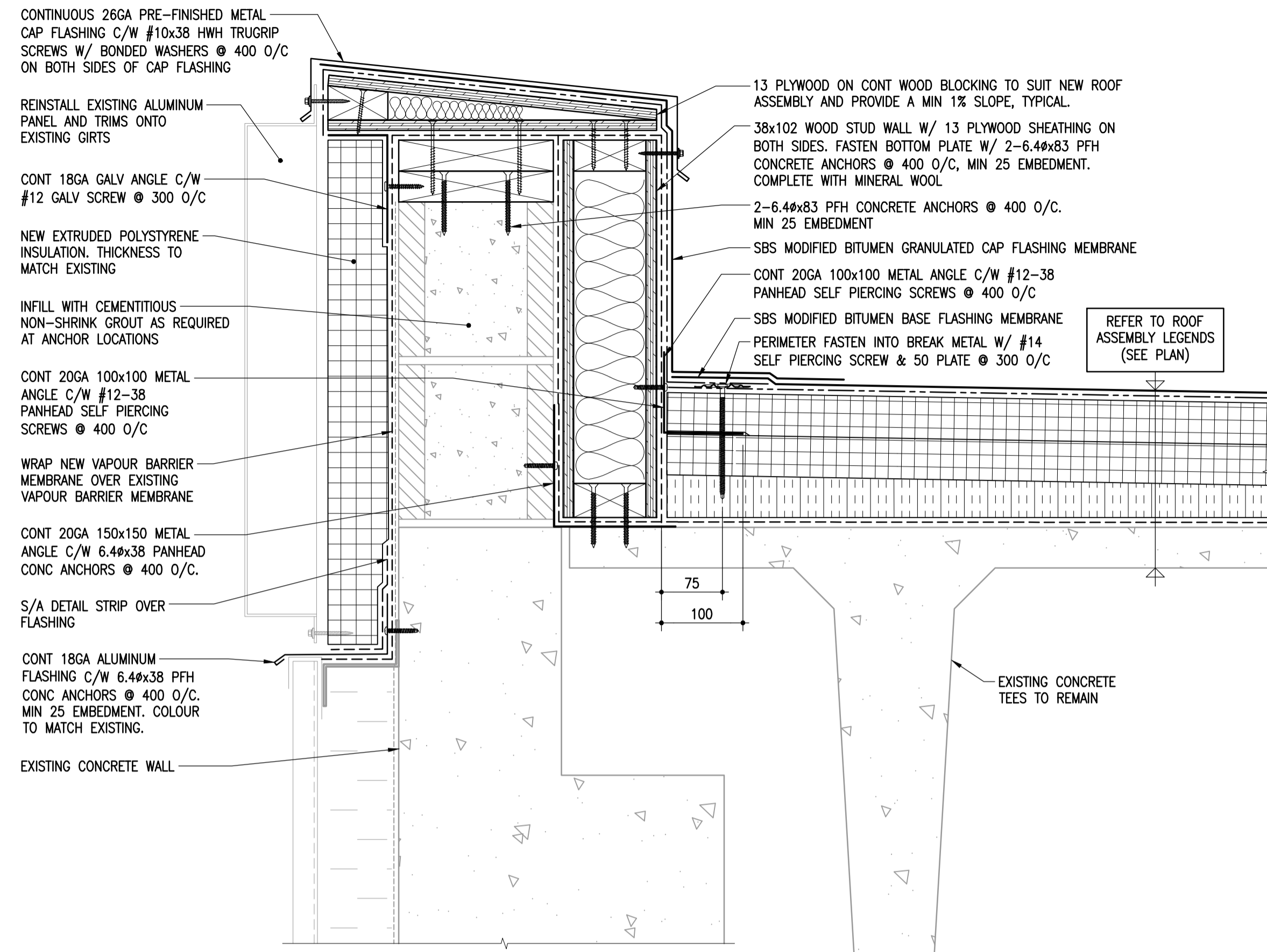
1 ROOF DETAIL AT CONCRETE TEE 1-0601B-80076-001 1:5
