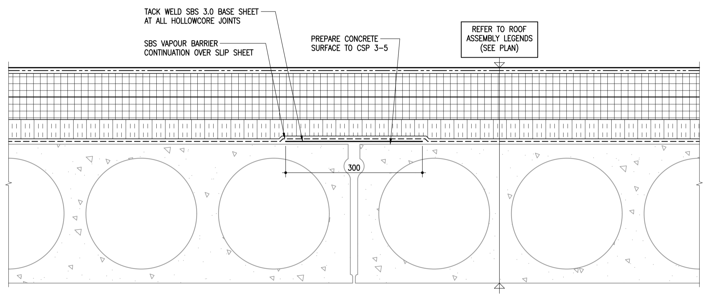
2 ROOF DETAIL AT HOLLOWCORE 1-0601B-80076-001 1:5
