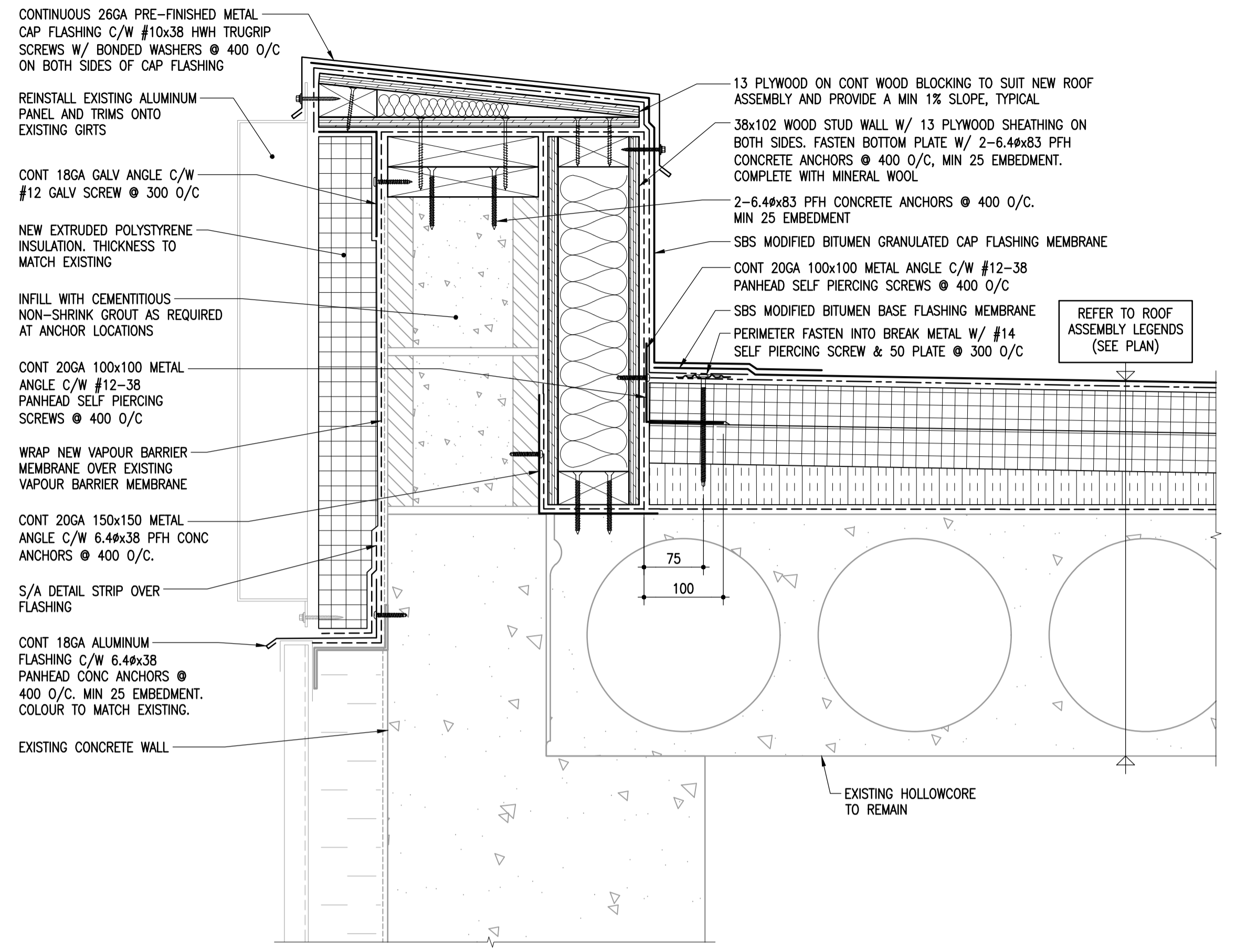
2 ROOF DETAIL AT HOLLOWCORE 1-0601B-80076-001 1:5
