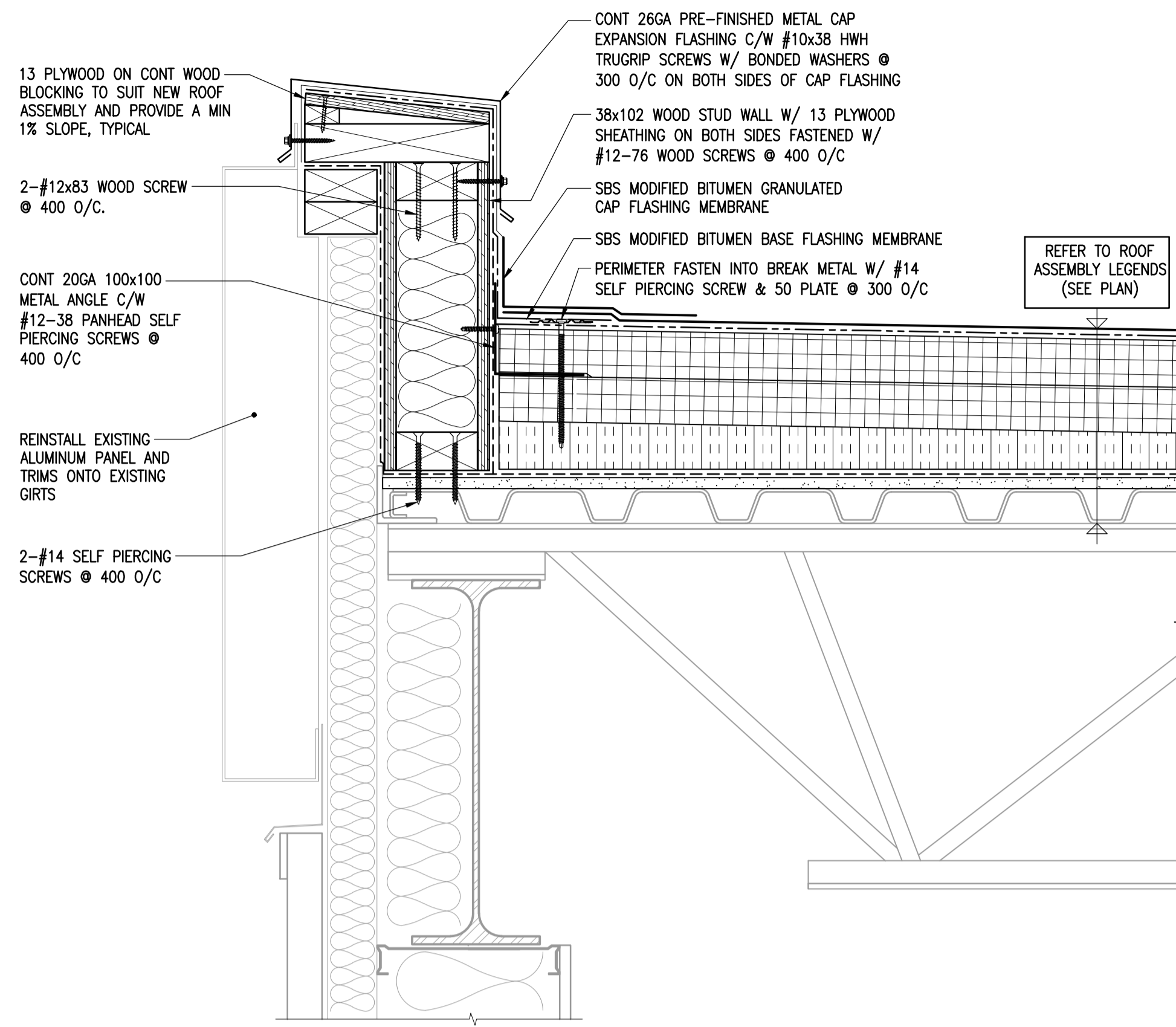
1 PARAPET ROOF DETAIL AT PENTHOUSE
