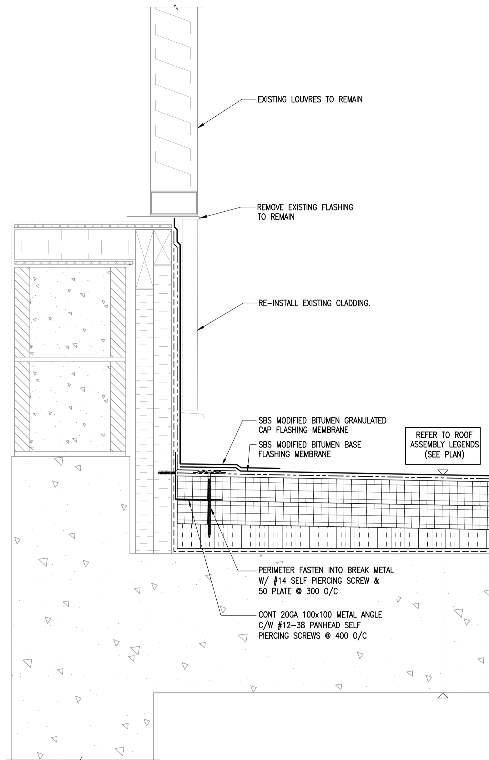
3 ROOFING TIE-IN DETAIL (AT LOUVRES)
