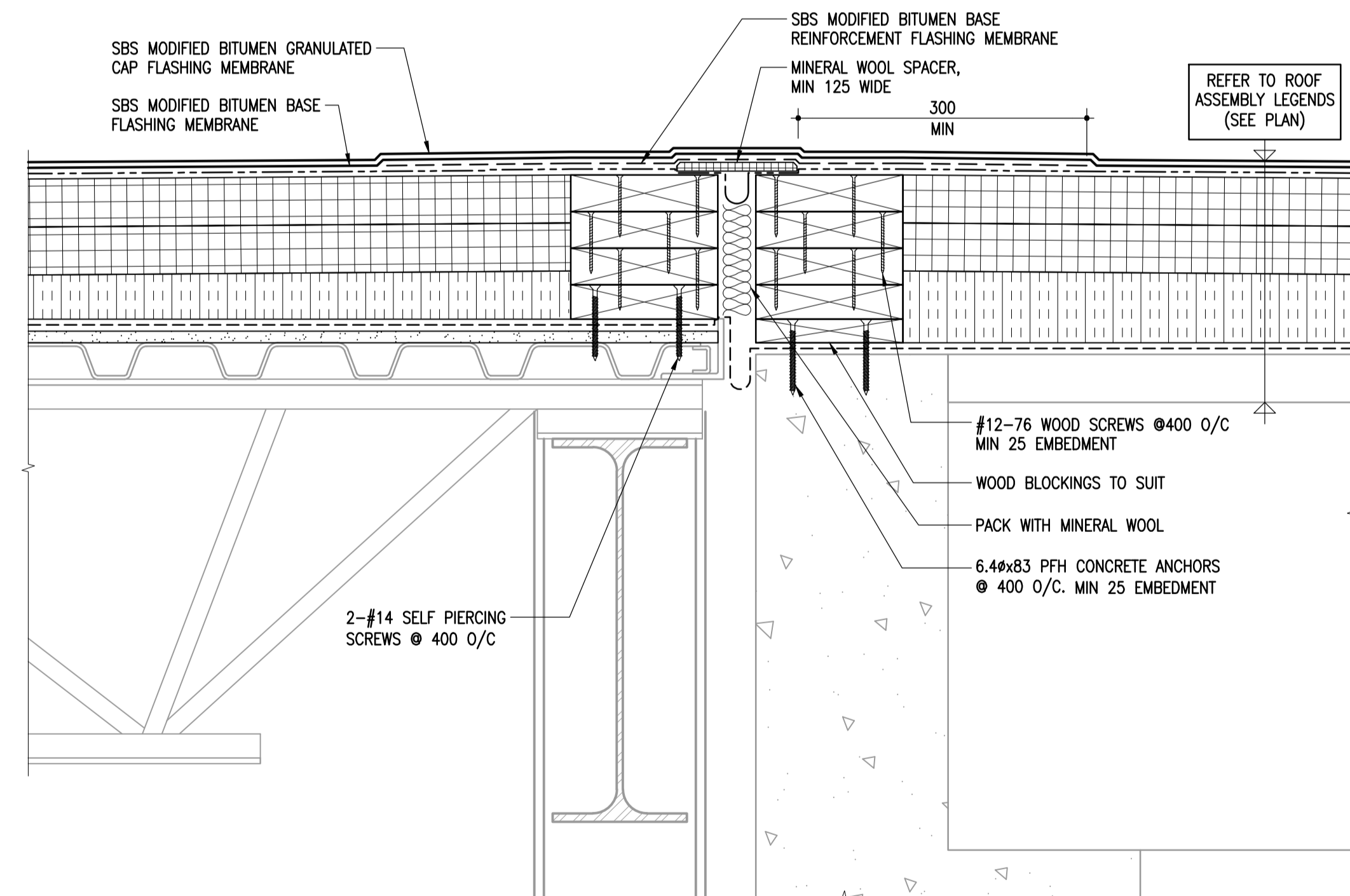
2 ROOF TIE-IN AT SAME ELEVATION
