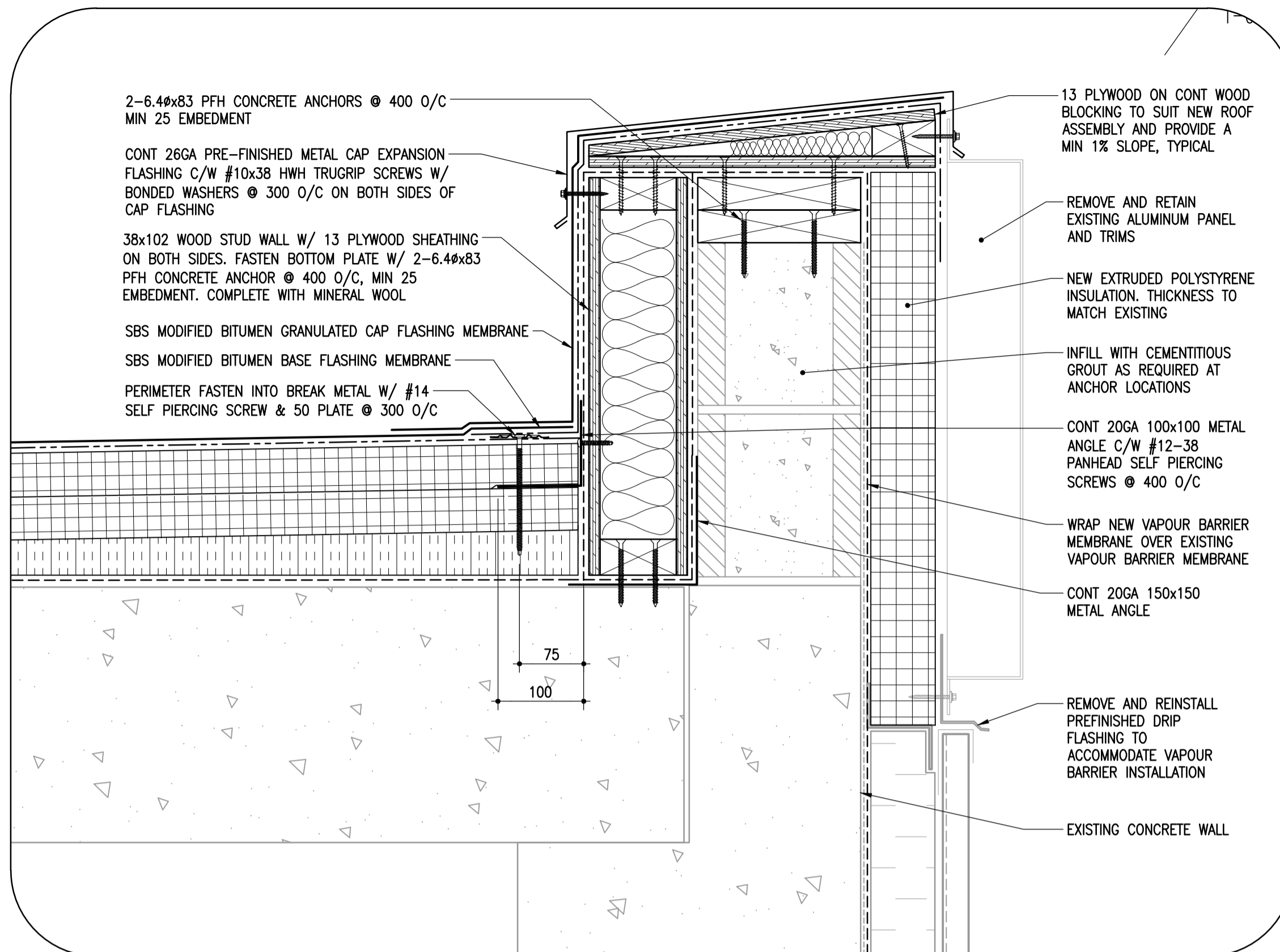
A PARAPET DETAIL 1-0601B-80076-006 1:5
