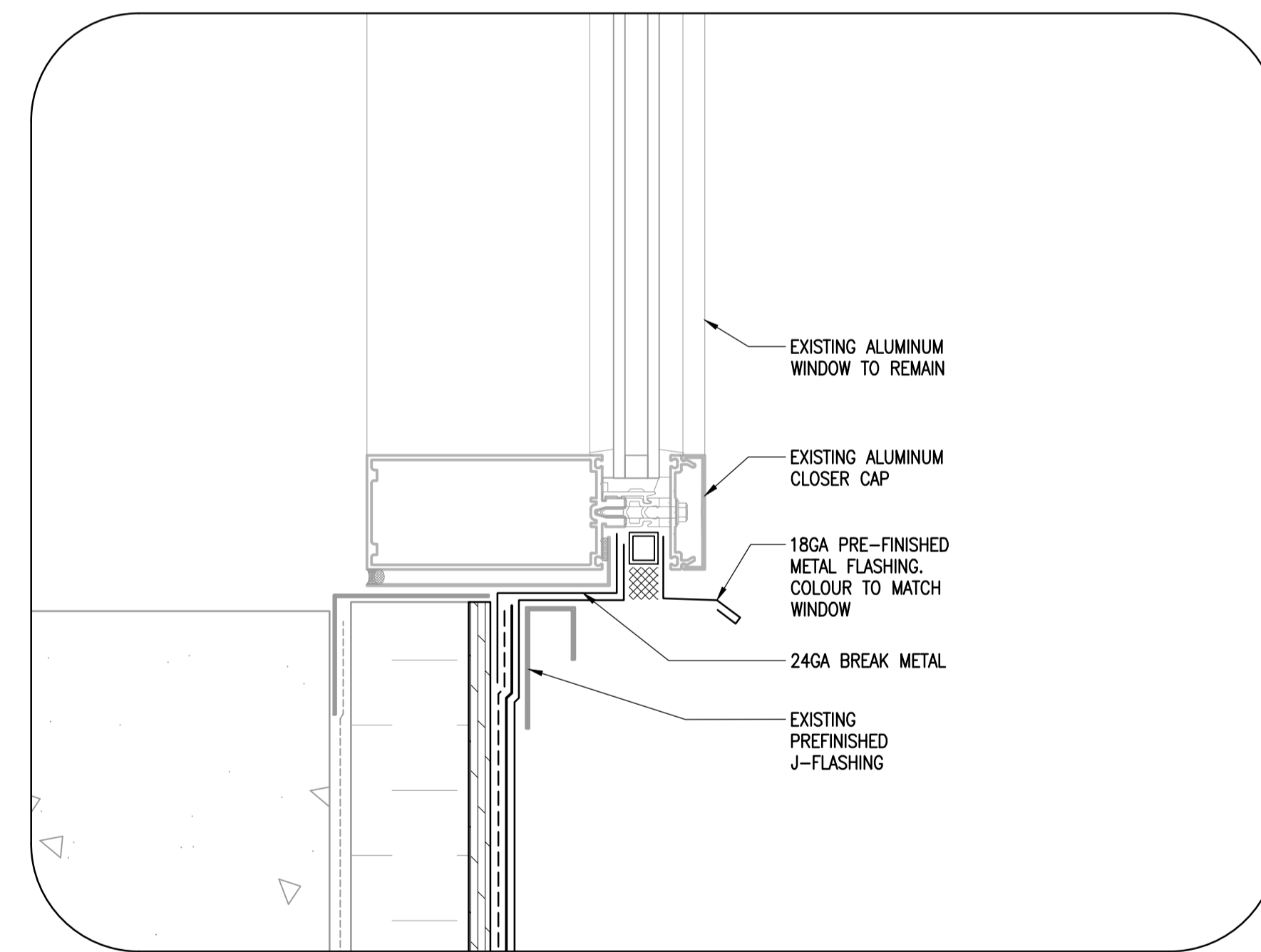
D CLERESTORY SILL DETAIL 1-0601B-80076-006 1:5
