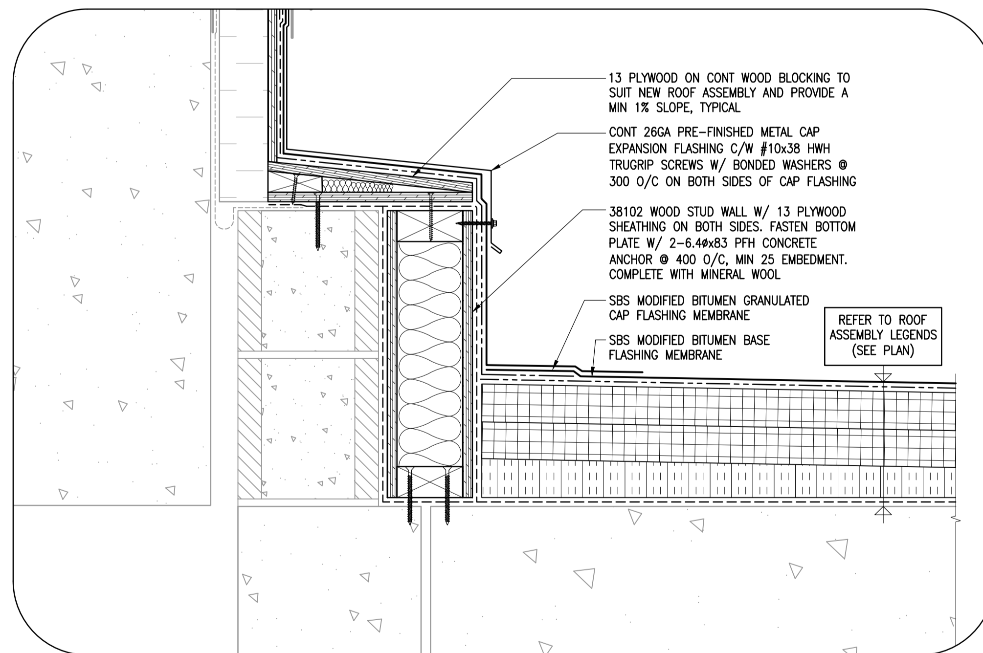
B WALL INTERFACE DETAIL 1-0601B-80076-006 1:5
