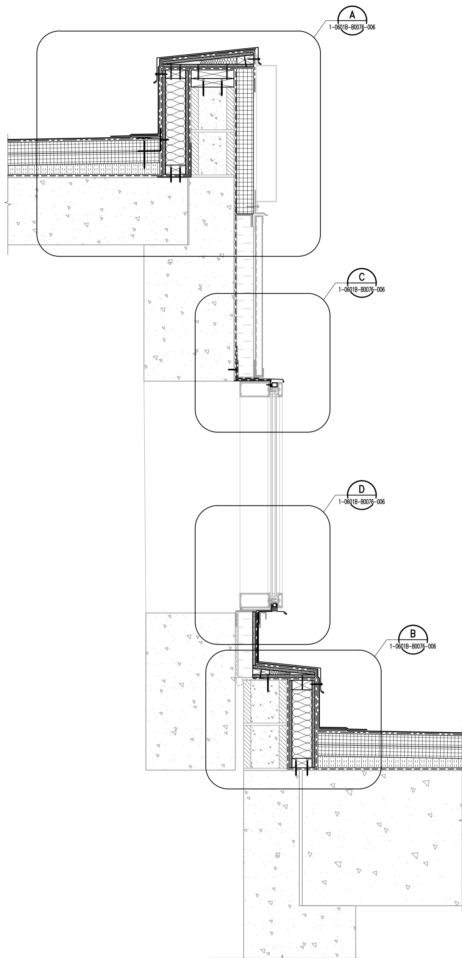
1 ROOF SECTION AT CLERESTORY 1-0601B-80076-006 1:10
