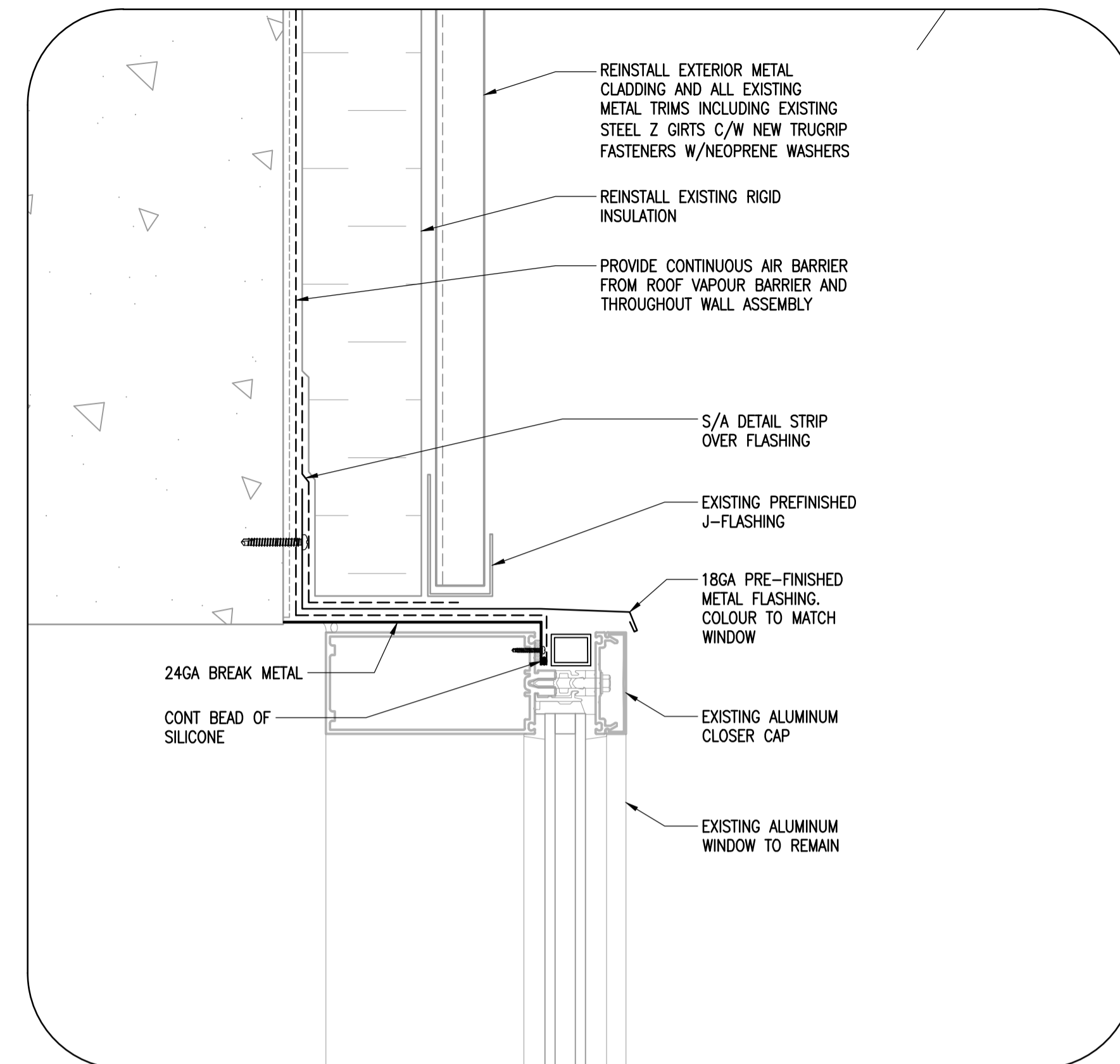
C CLERESTORY HEAD DETAIL 1-0601B-80076-006 1:5
