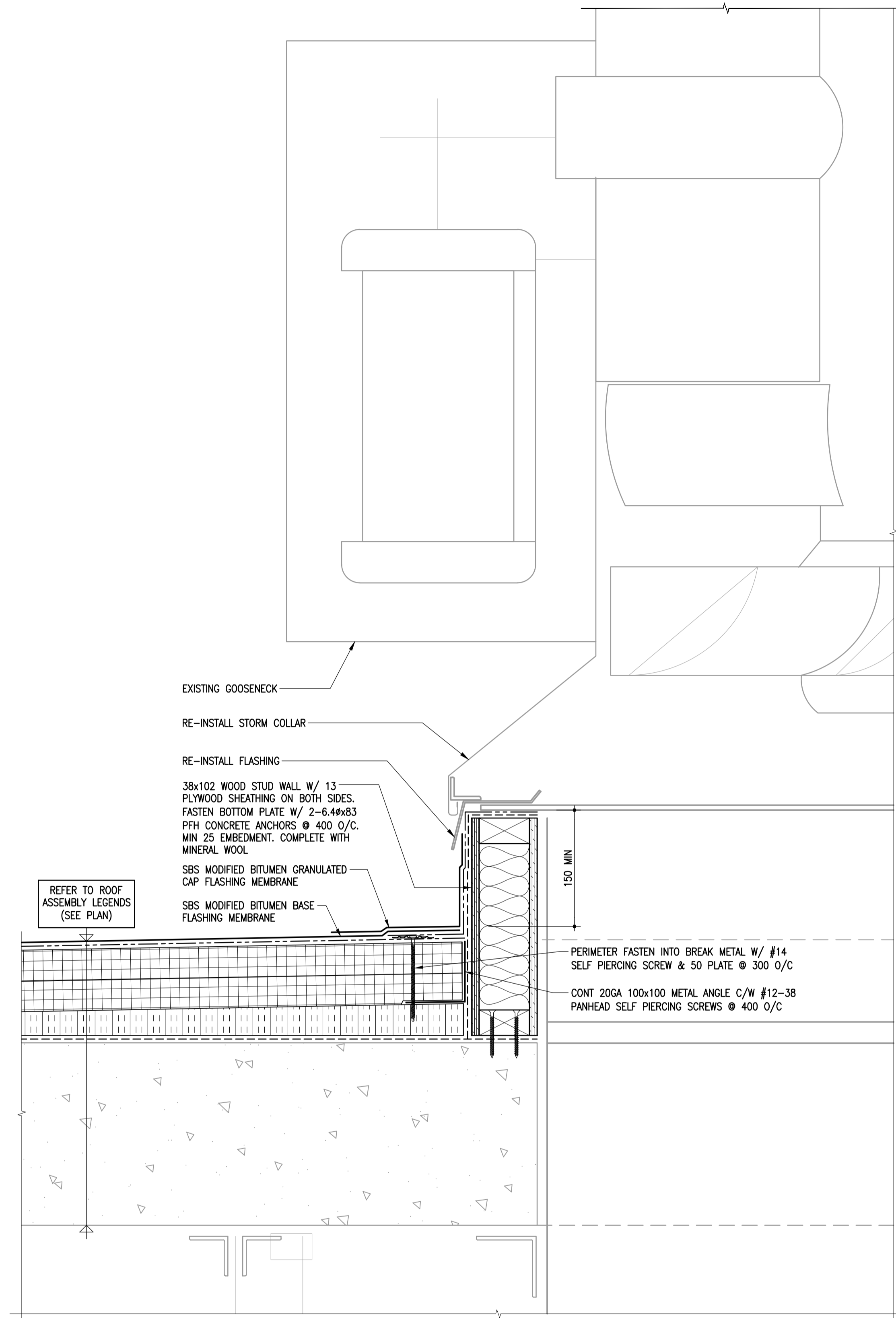
1 GOOSENECK DETAIL 1-0601B-00076-008 1:5
