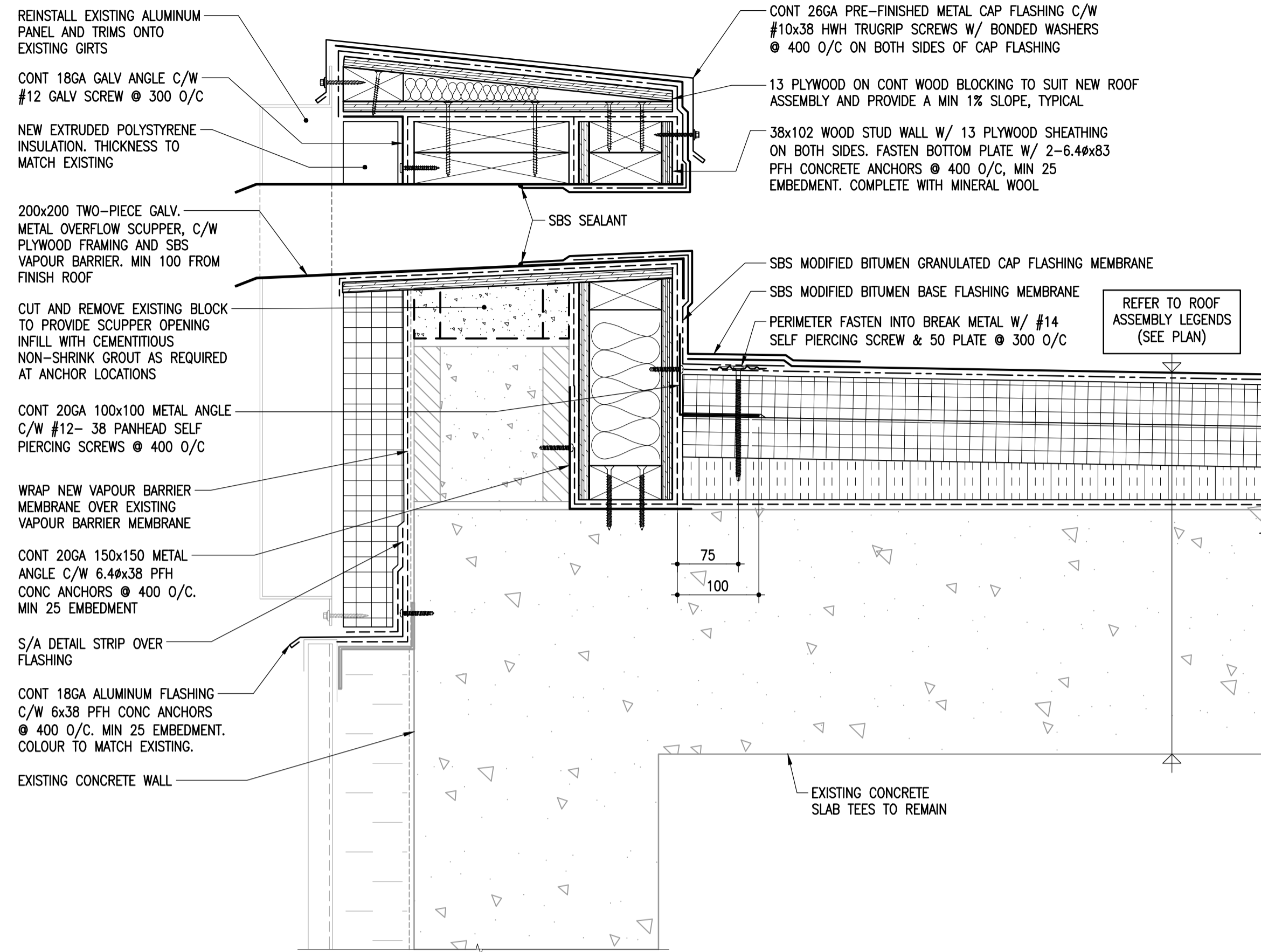
1 OVERFLOW SCUPPER DETAIL 1-0601B-0076-09 1:5
