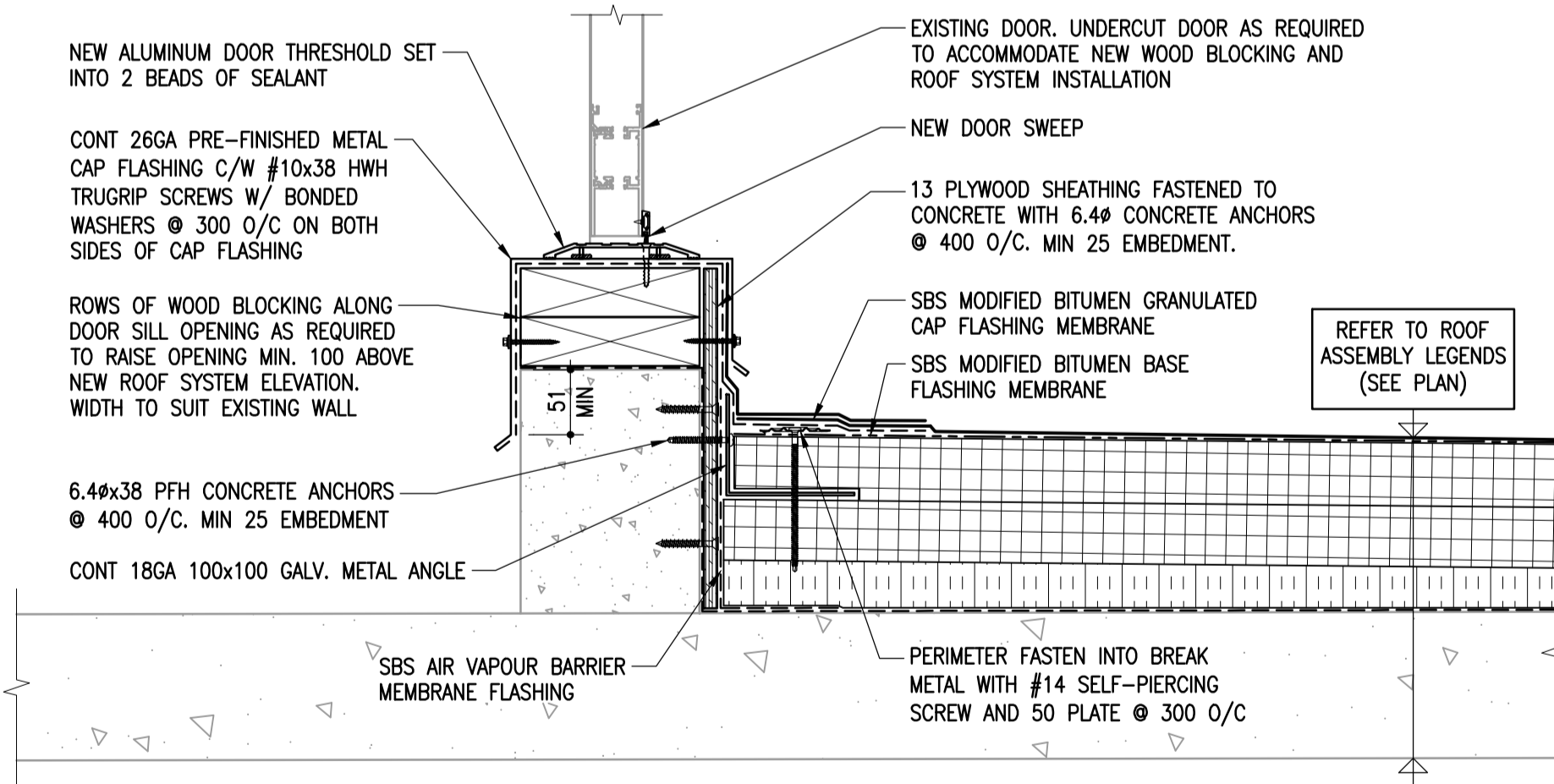
2 ROOF DETAIL AT ACCESS DOOR 1-0601B-0076-09 1:5
