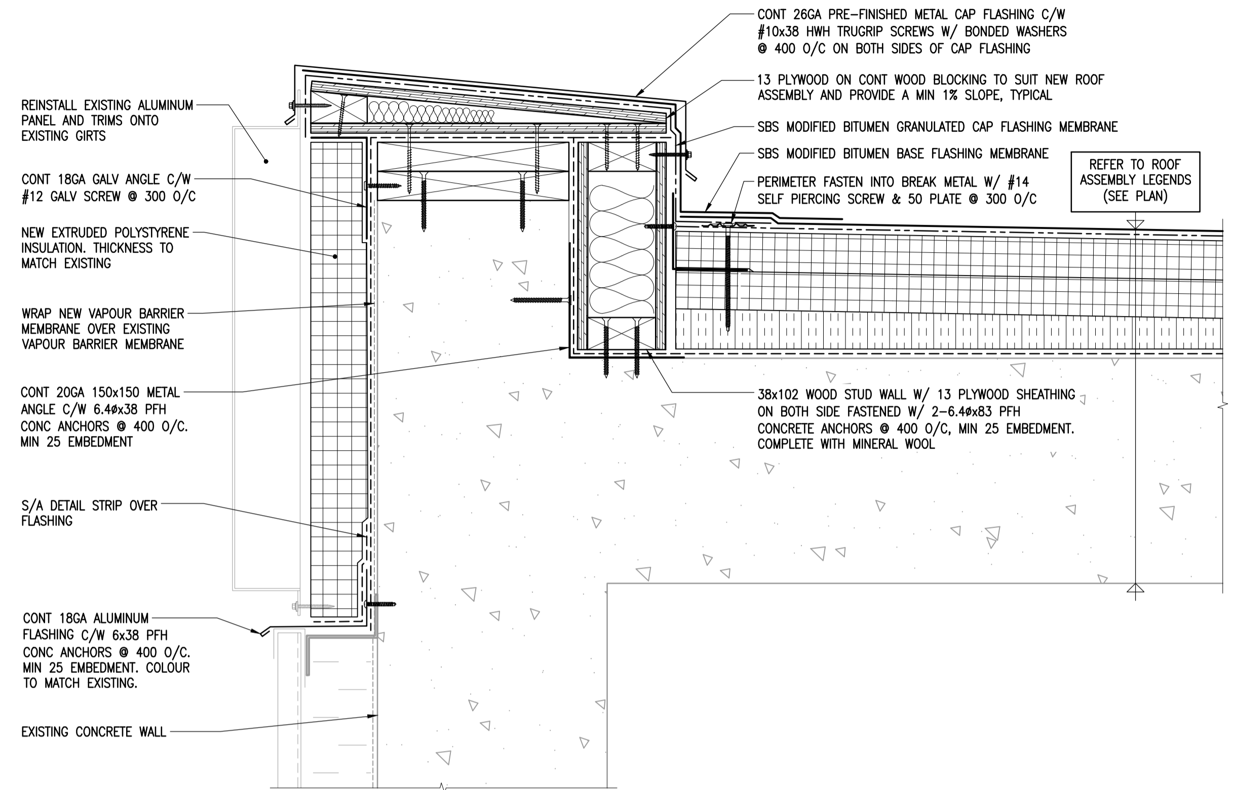
3 ROOFING TIE-IN DETAIL 1-0601B-0076-09 1:5
