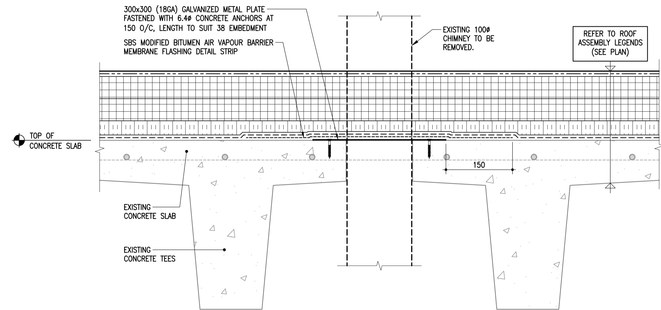
4 THRU SLAB INFILL DETAIL 1-0601B-0076-09 NTS
