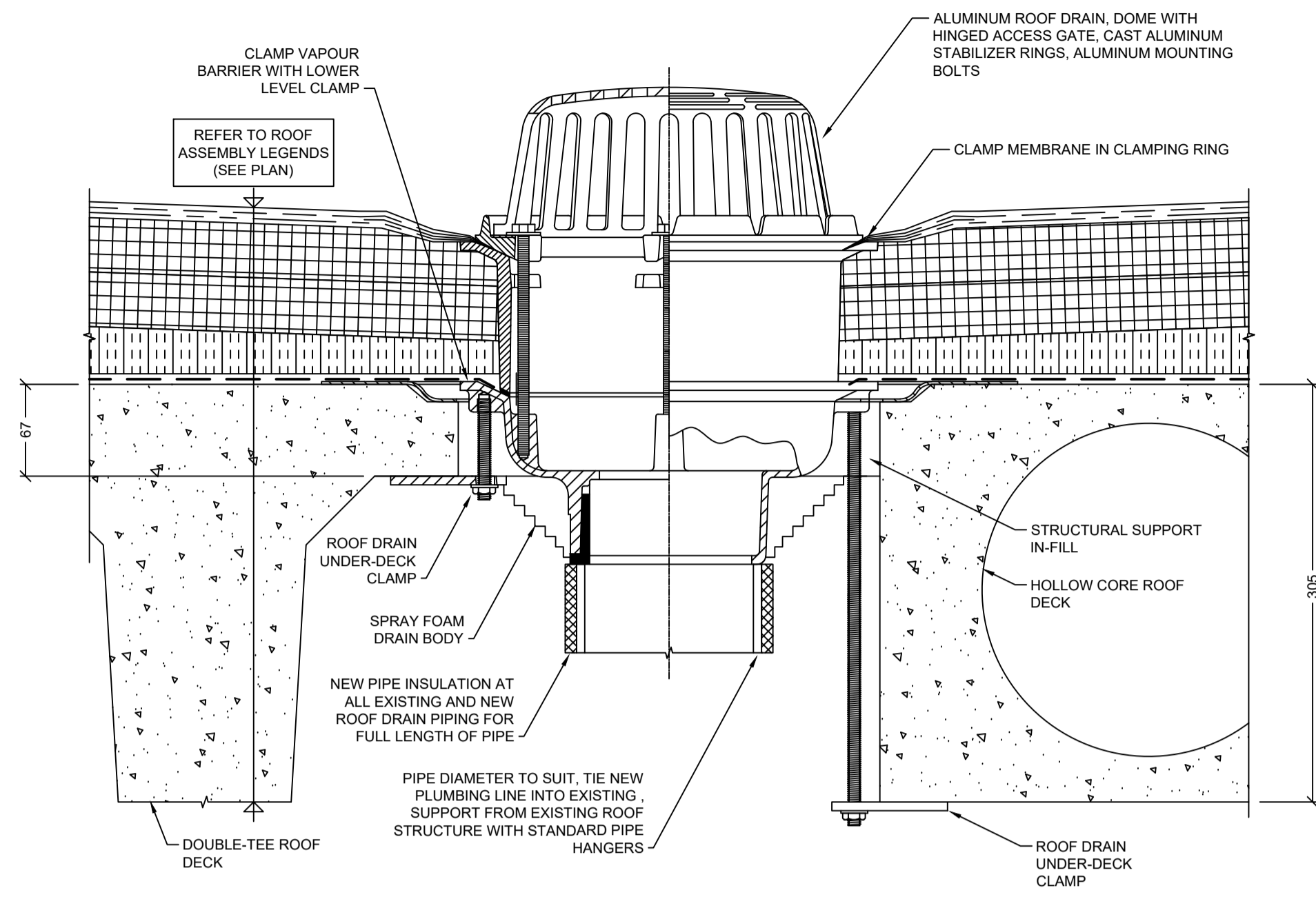
1 PRIMARY ROOF DRAIN: RD-1 SCALE: NTS M3.3
