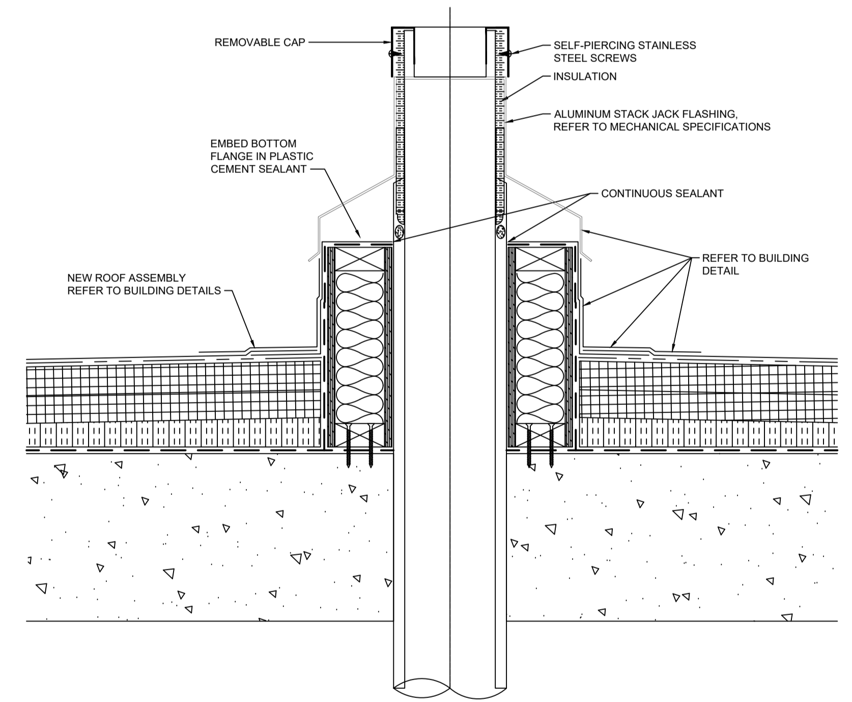
5 PLUMBING VENT THROUGH ROOF SCALE: NTS M3.3
