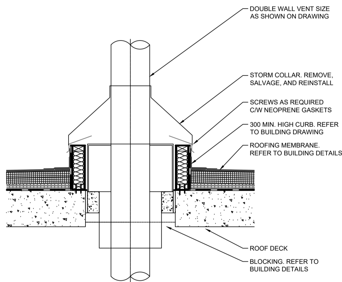
3 CHIMNEY THROUGH ROOF SCALE: NTS M3.3
