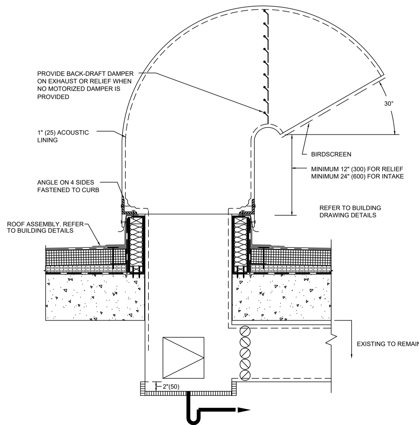
4 INTAKE OR OUTLET AIR GOOSENECK SCALE: NTS M3.3
