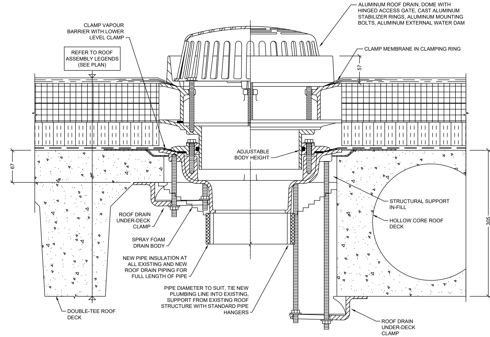
2 OVERFLOW ROOF DRAIN: RD-2 SCALE: NTS M3.3
