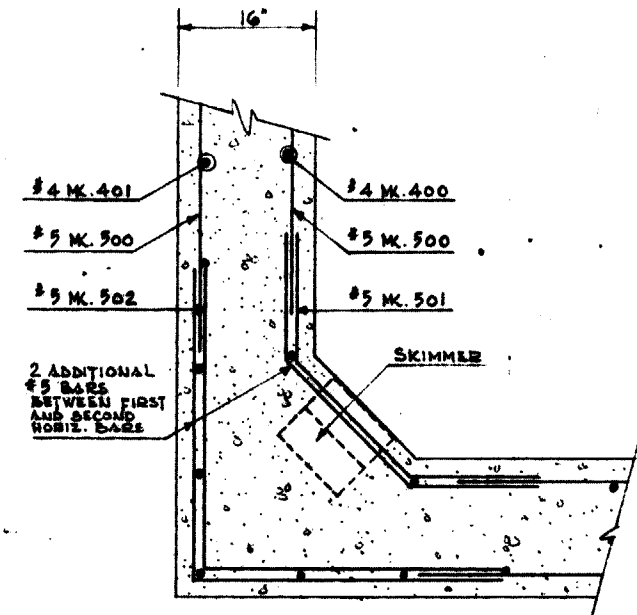
CORNER DETAIL
