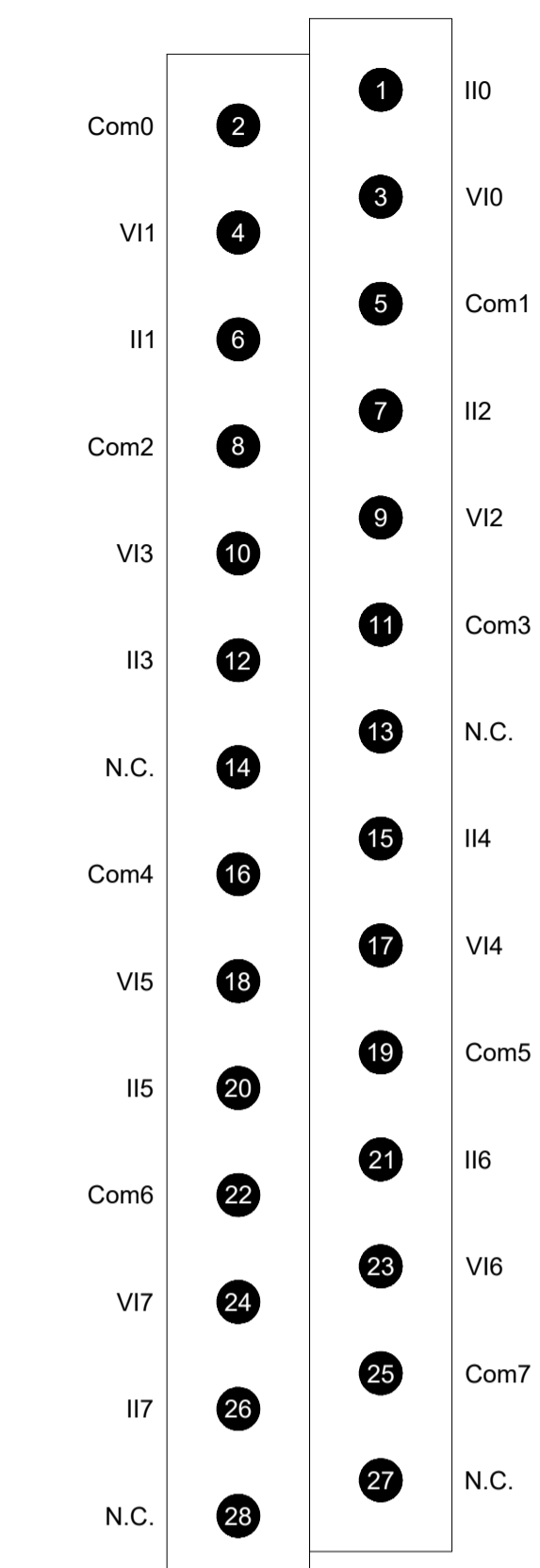
PINOUT DIAGRAM
