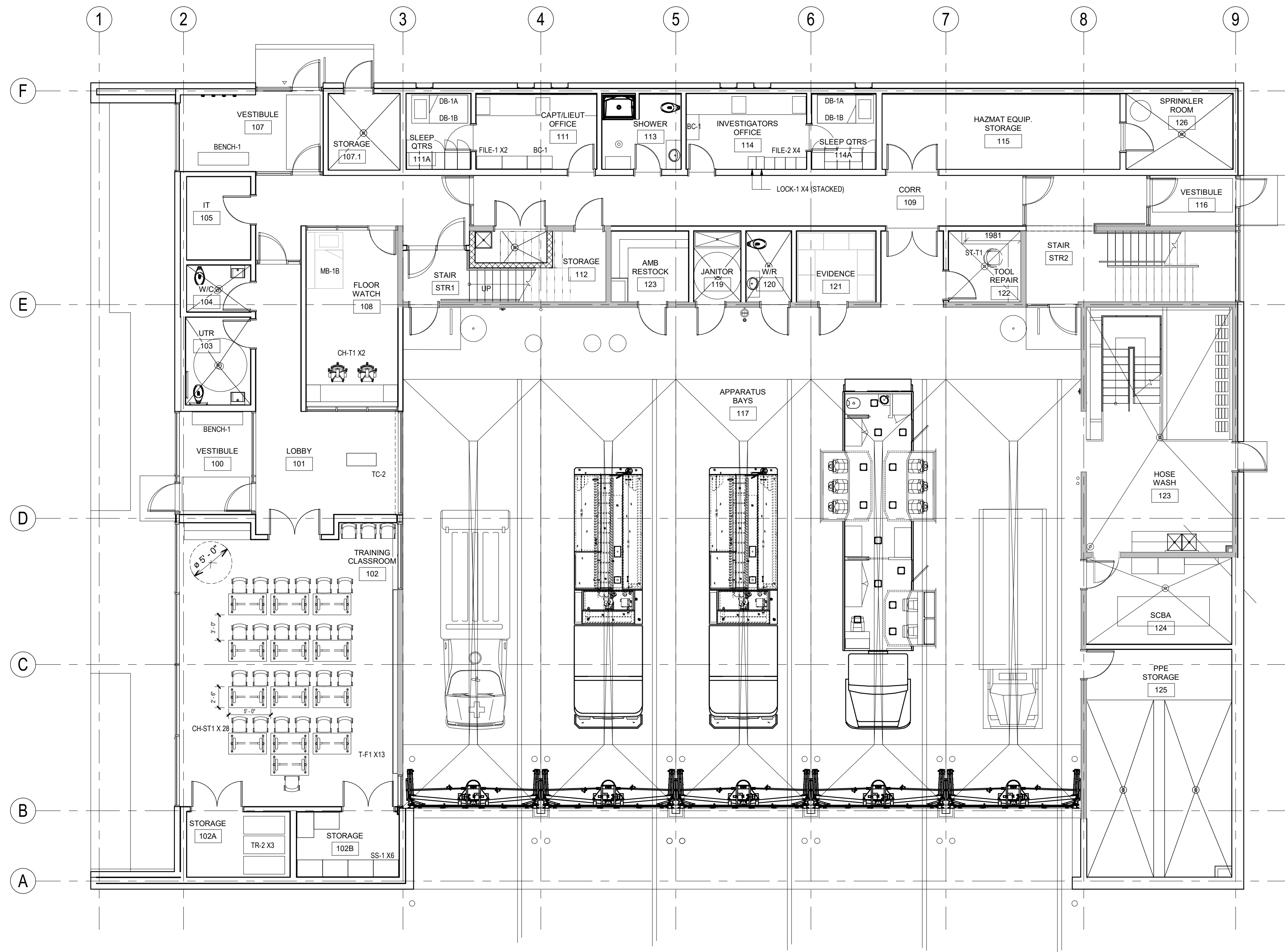
1 FURNITURE PLAN - MAIN FLOOR A800 1/8" = 1'-0"
