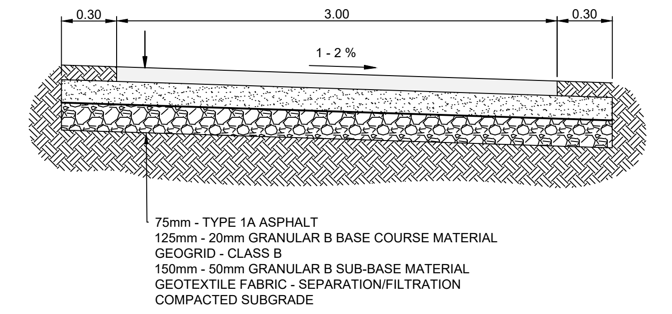
CROSS SECTION "A" - ASPHALT RECONSTRUCTION N.T.S
