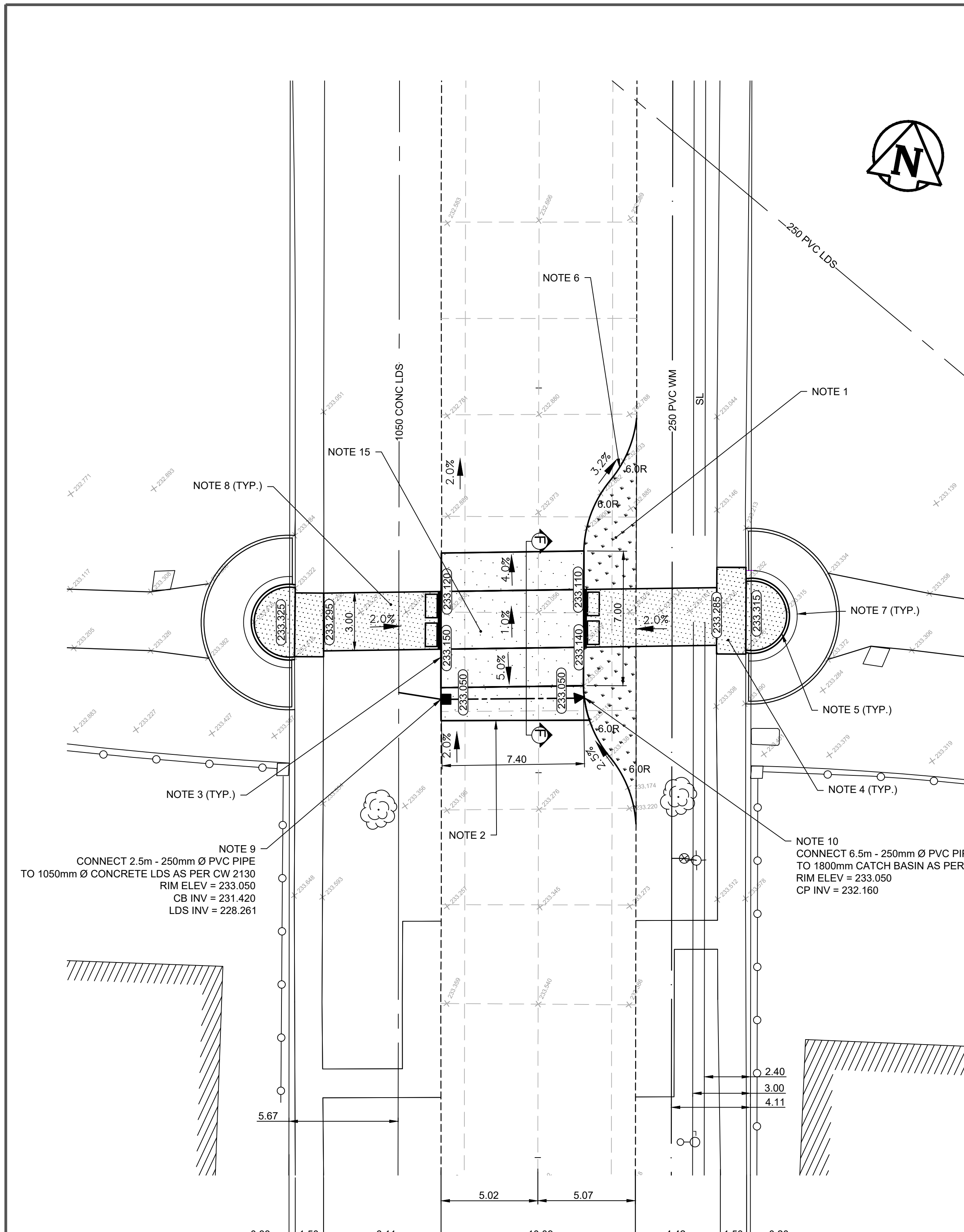
DETAIL A SCALE 1:150
