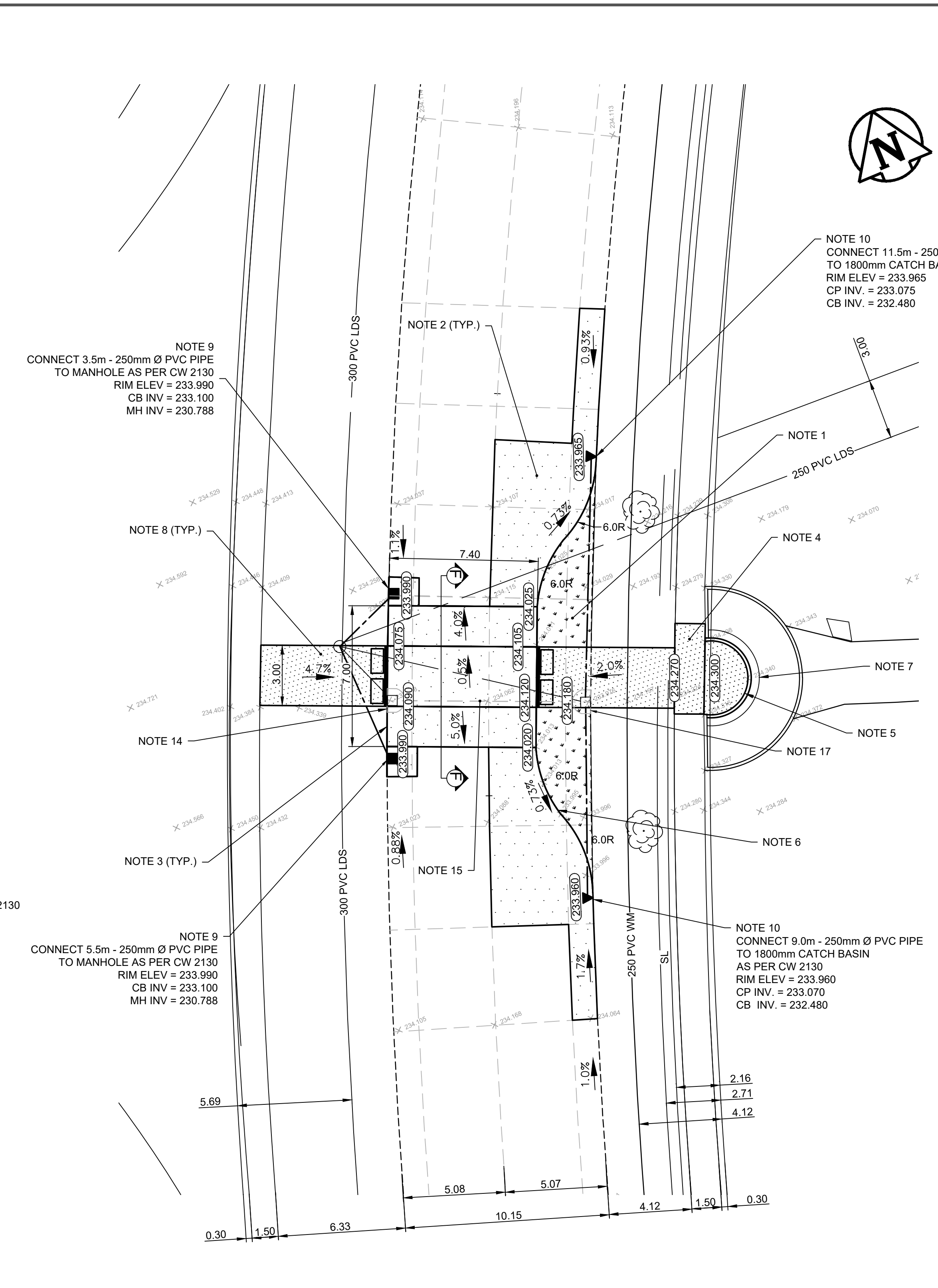
DETAIL B SCALE 1:150
