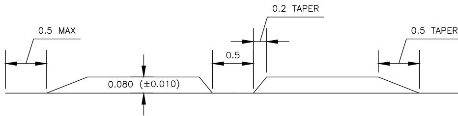
SECTION C-C
