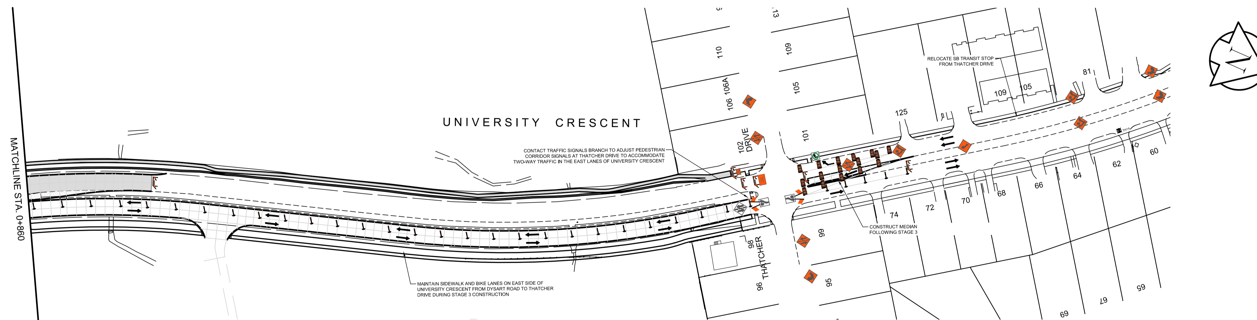
PLAN - TRAFFIC DETOUR STAGE 3 Scale 1:1000
