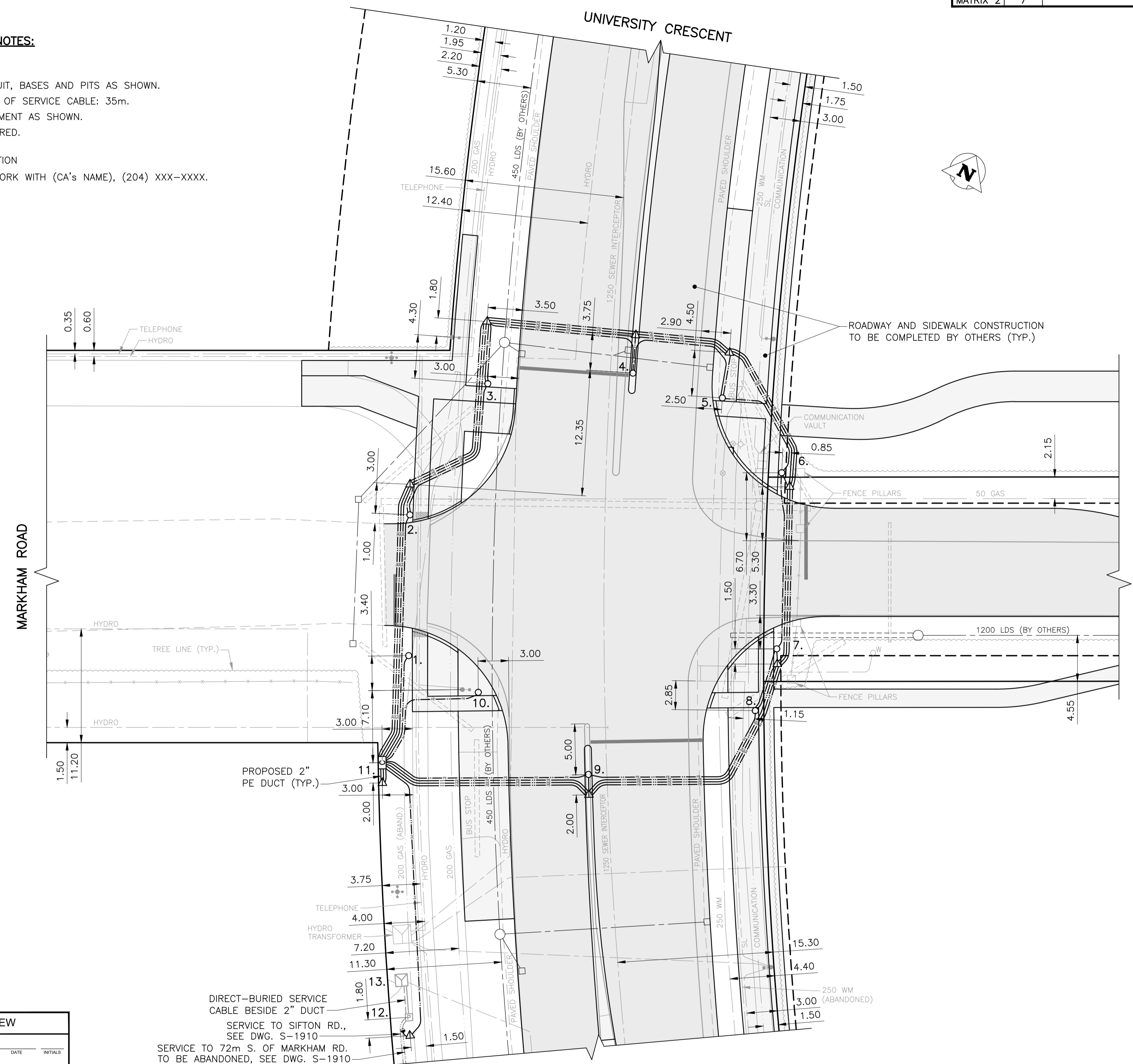
PLAN VIEW: UNDERGROUND CONSTRUCTION 1:250
