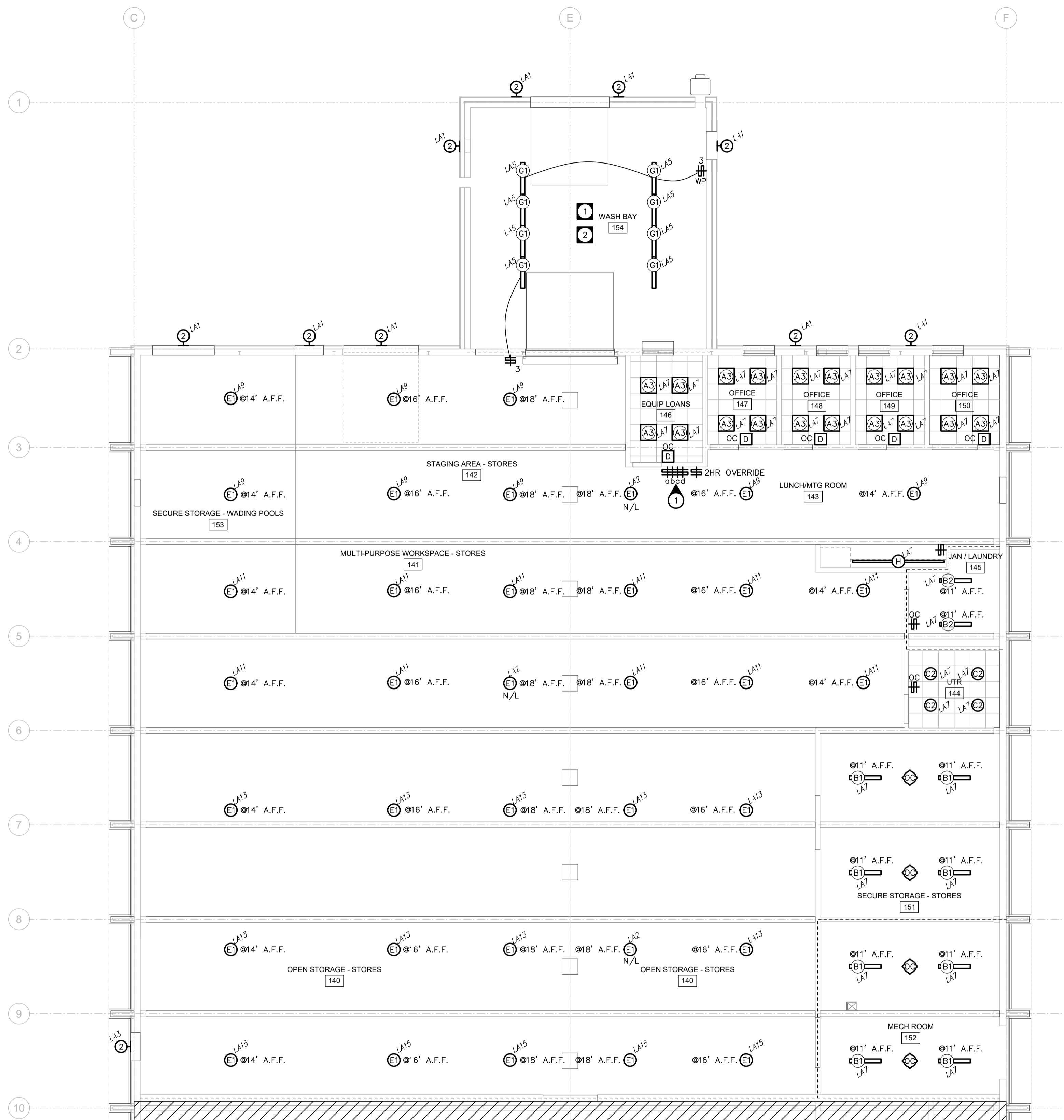
1 LIGHTING LAYOUT - NORTH AREA E3.0 SCALE: 1/100
