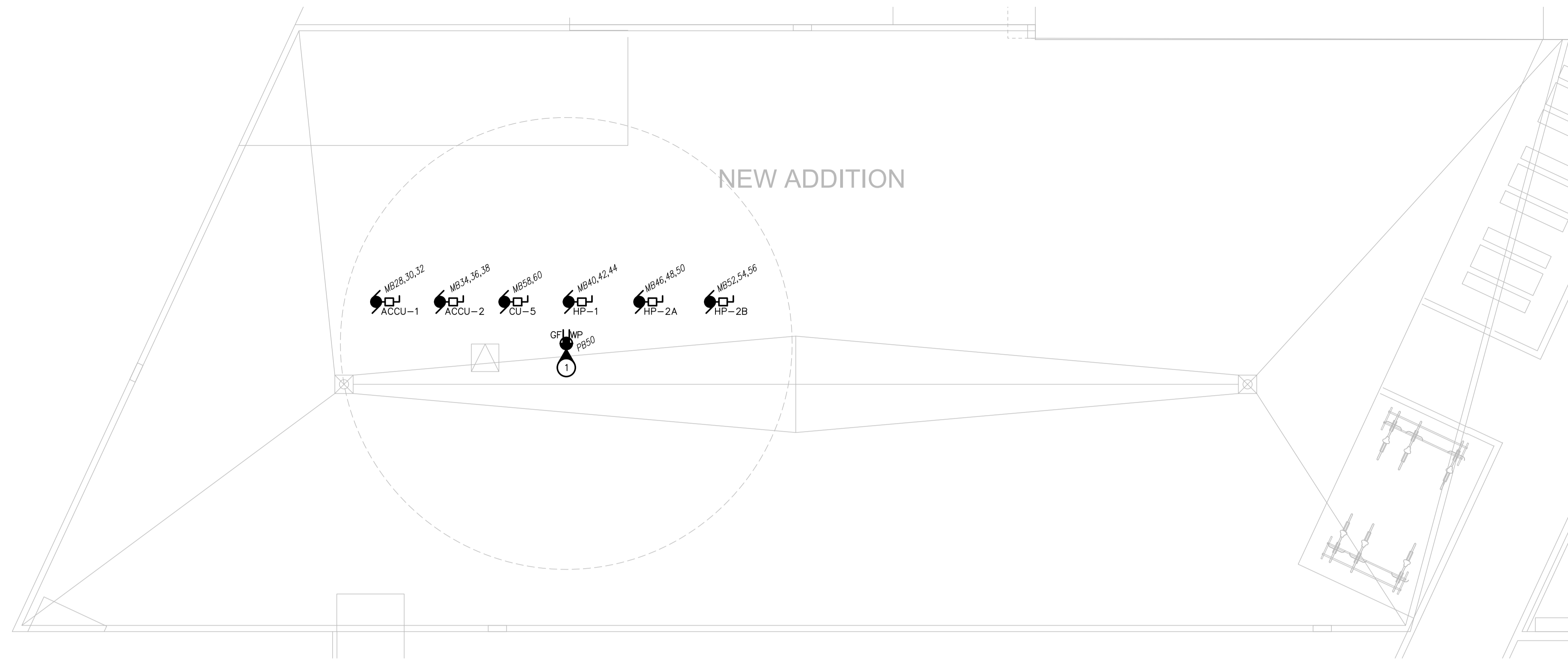
1 POWER LAYOUT - ROOF PLAN E4.2 SCALE: 1:100
