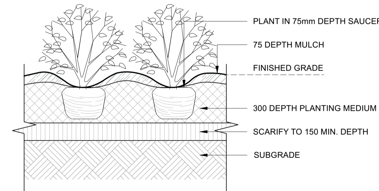
6 L2.4 NIC - WORK BY OTHERS SHRUB PLANTING Scale: 1:20
