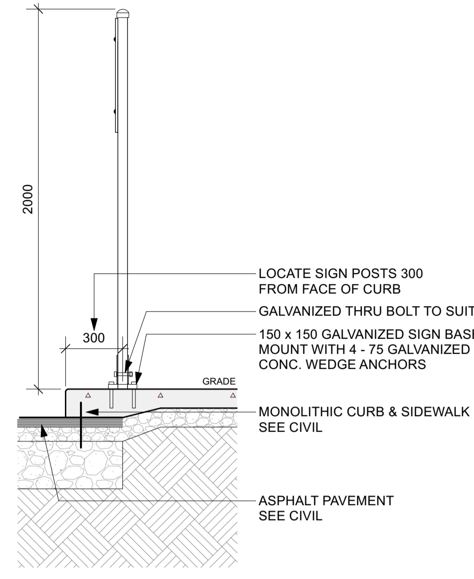
2B L2.4 SIGN POST SURFACE MOUNT
