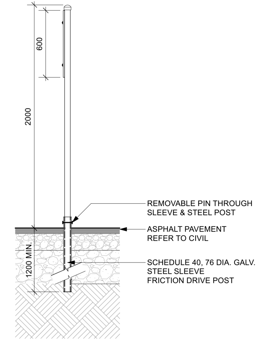
2D L2.4 SIGN POST IN ASPHALT
