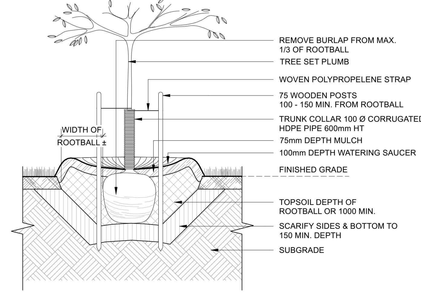
5 L2.4 NIC - WORK BY OTHERS DECIDUOUS TREE PLANTING Scale: 1:20
