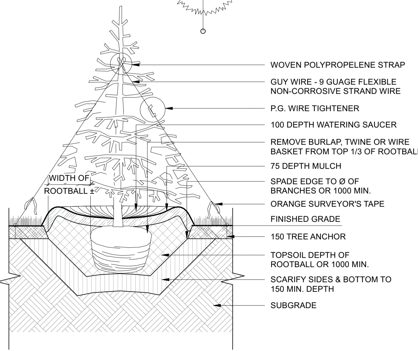
4 L2.4 NIC - WORK BY OTHERS CONIFEROUS TREE PLANTING Scale: 1:20
