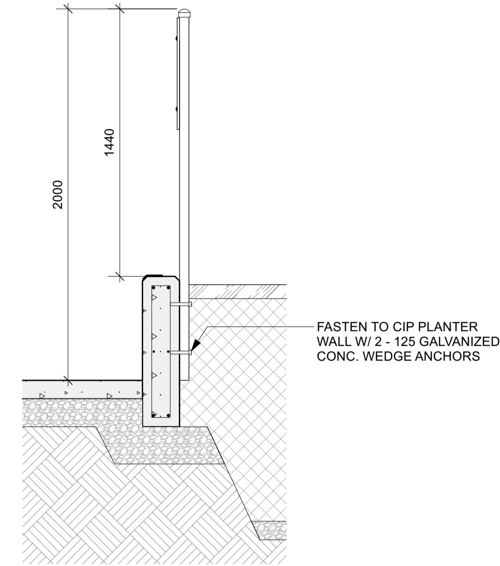
2C L2.4 SIGN POST WALL MOUNT
