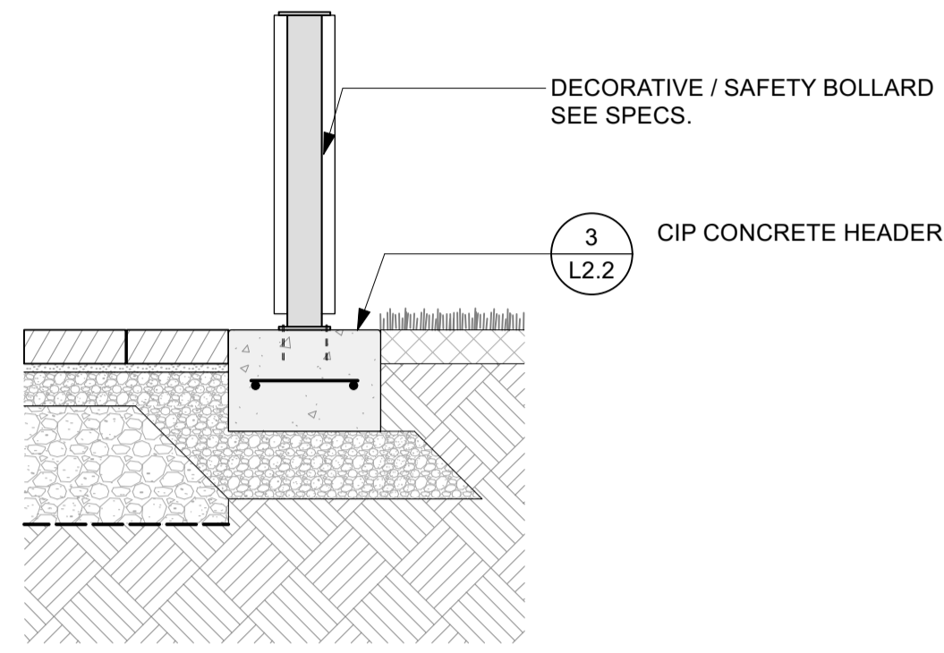
1 L2.4 DECORATIVE/SAFETY BOLLARD Scale: 1:20
