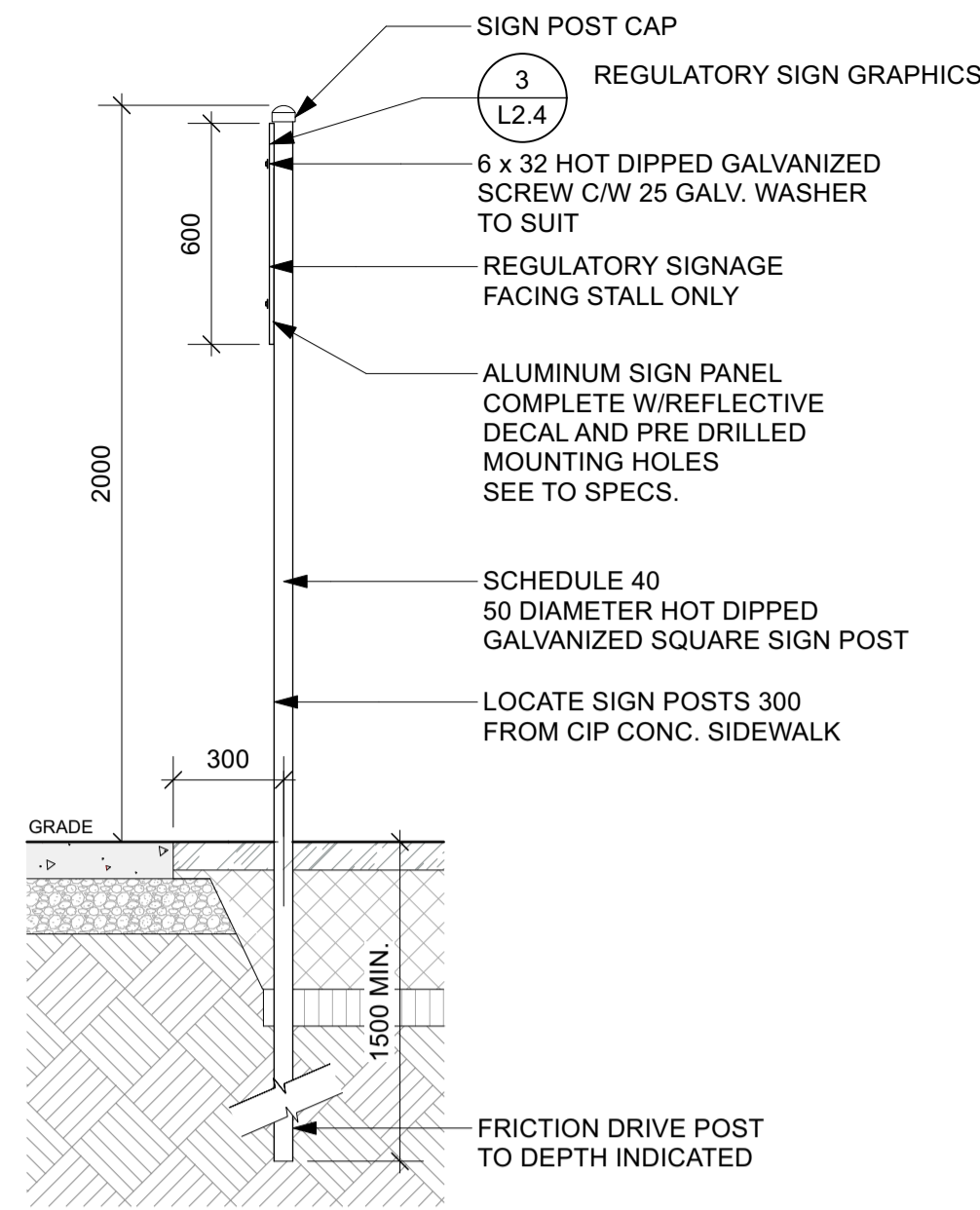
2A L2.4 SIGN POST IN SOFTSCAPE Scale: 1:20
