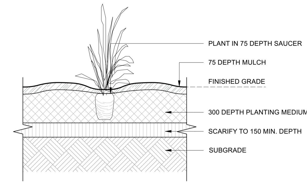
7 L2.4 NIC - WORK BY OTHERS PERENNIAL PLANTING Scale: 1:20
