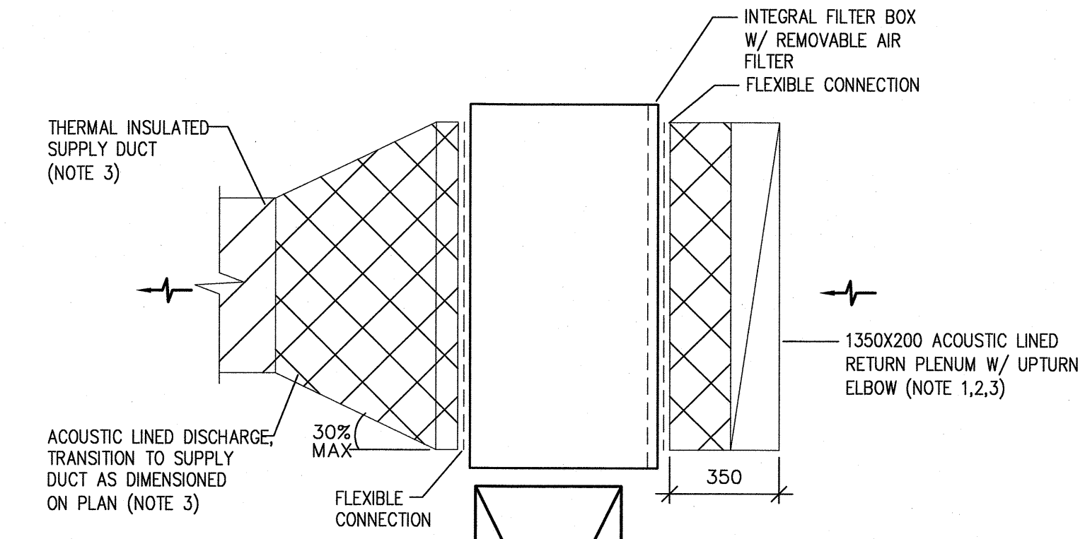
FAN COIL DUCT CONNECTIONS TYPICAL SIZE 24, 27, 30 N.T.S.
