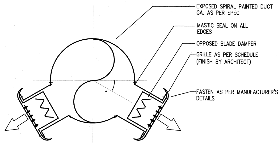
DIFFUSER INSTALLATION
