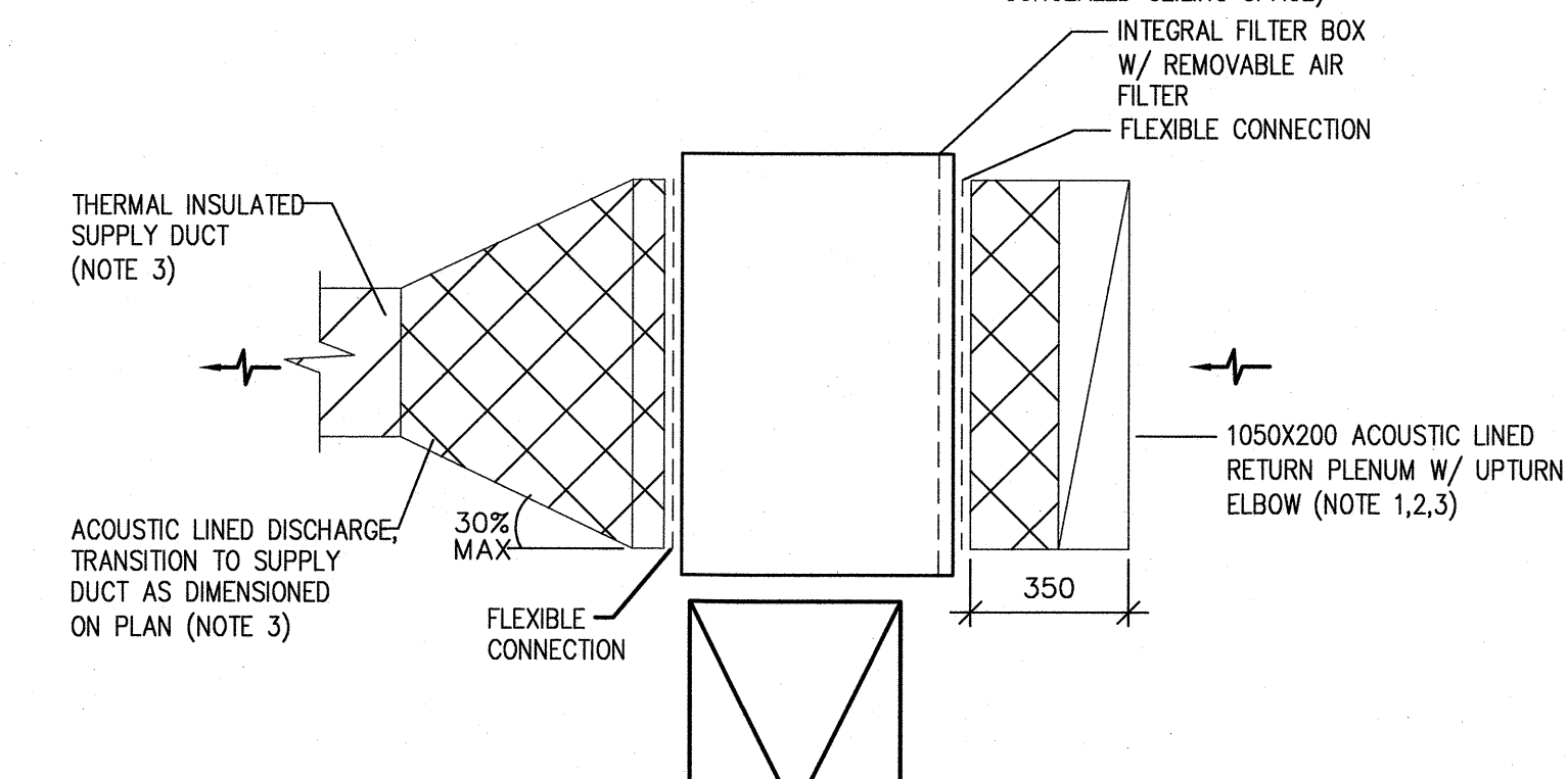
FAN COIL DUCT CONNECTIONS TYPICAL SIZE 15, 18 N.T.S.
