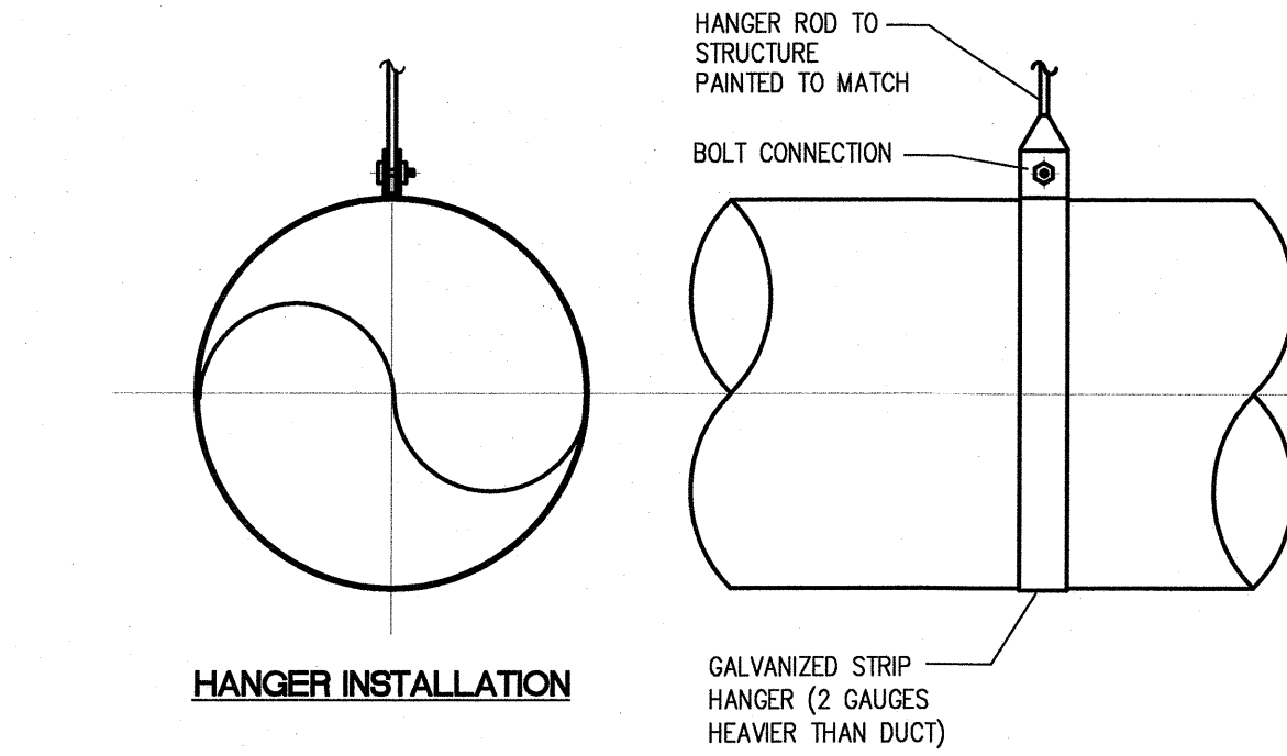
TYPICAL EXPOSED ROUND DUCT INSTALLATION N.T.S.
