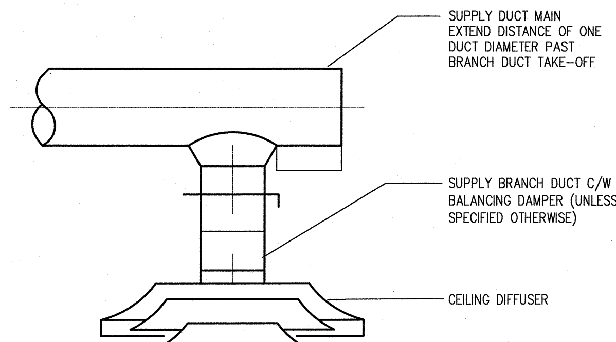
TYPICAL EXPOSED ROUND DUCT INSTALLATION N.T.S.
