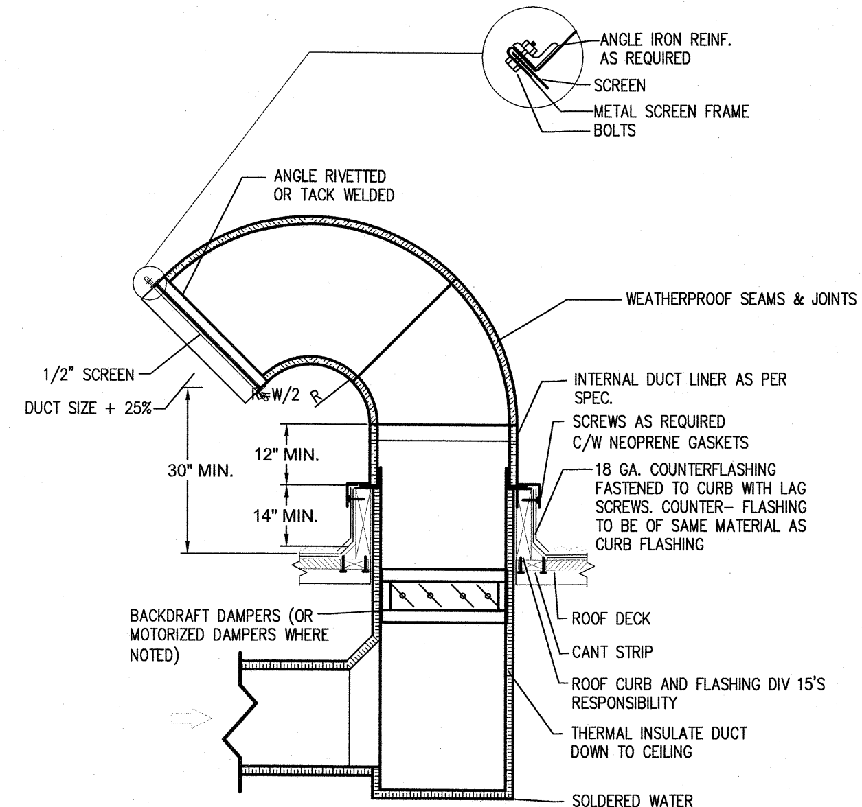
RECTANGULAR EXHAUST GOOSENECK DETAIL N.T.S.
