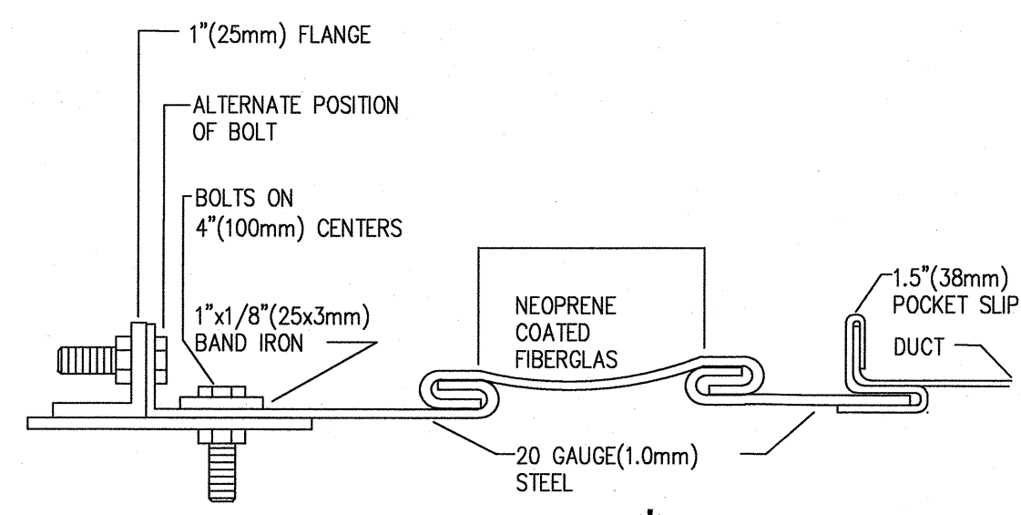
DUCT CONNECTION DETAILS N.T.S.
