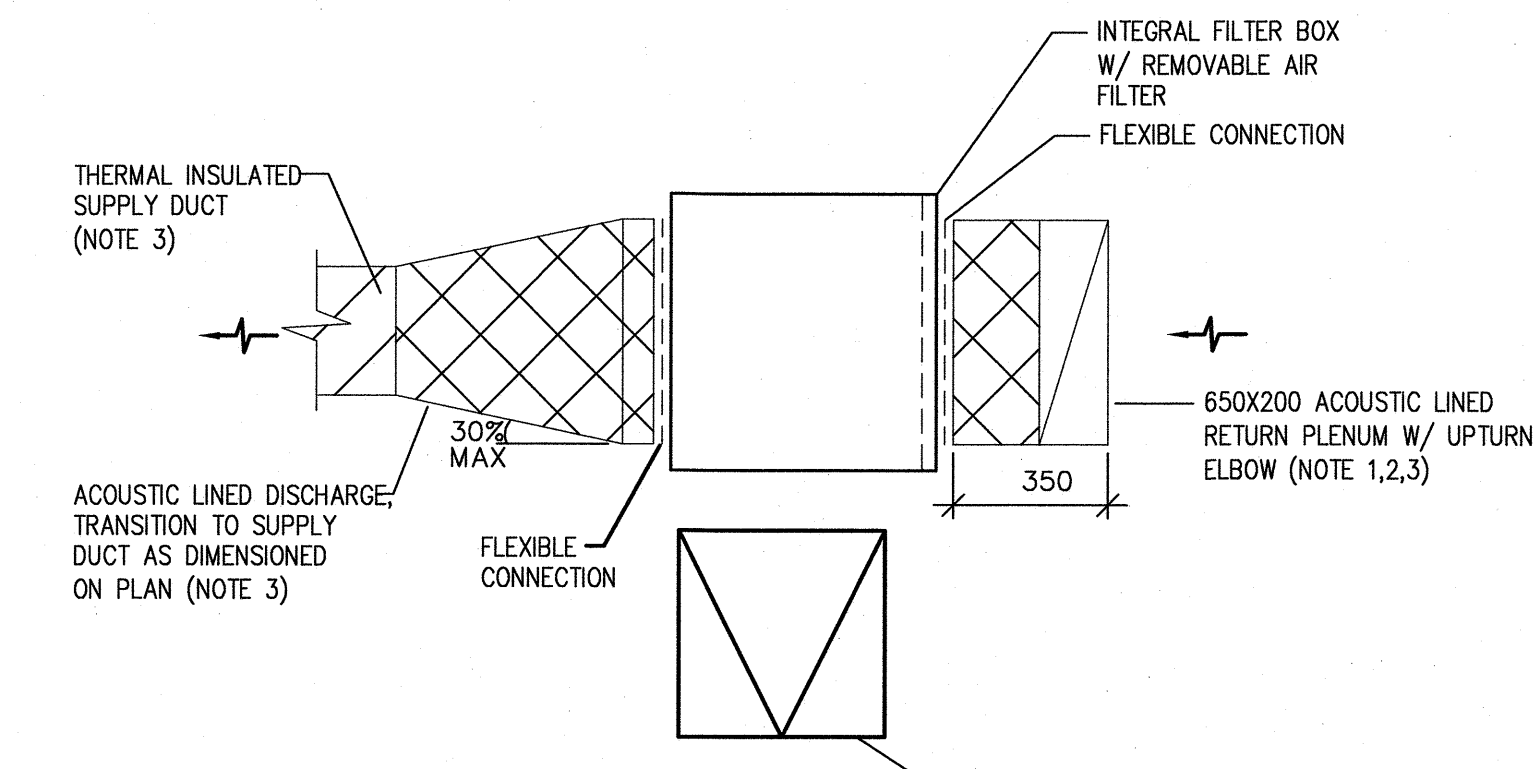
FAN COIL DUCT CONNECTIONS TYPICAL SIZE 06, 08, 12 N.T.S.
