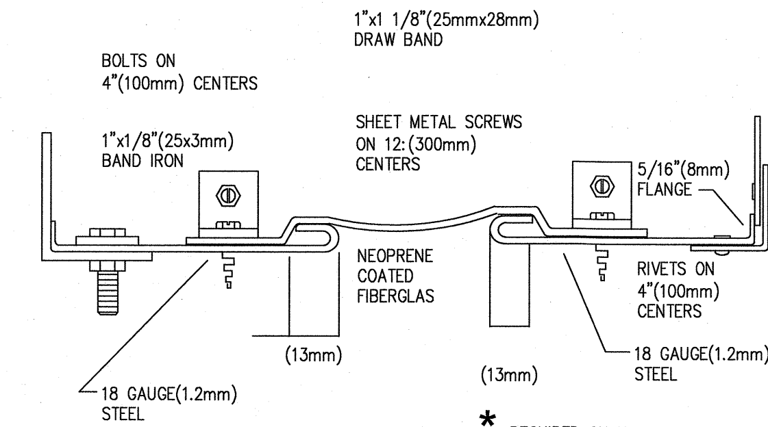
DUCT CONNECTION DETAILS N.T.S.
