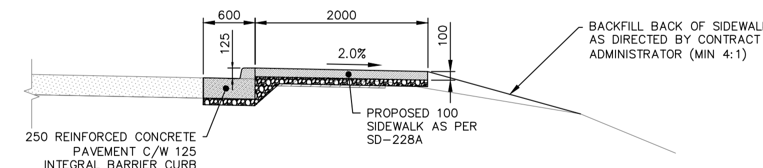
DETAIL "A" - MONOLITHIC CURB AND SIDEWALK WITH PAVEMENT WIDENING NTS
