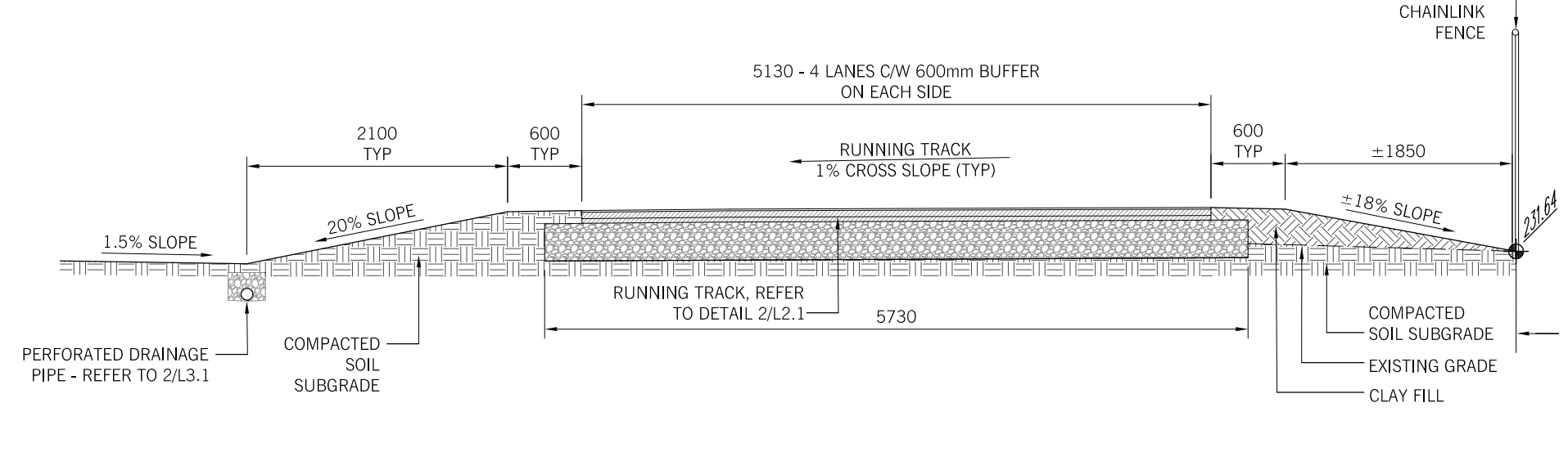
4 SECTION THROUGH TRACK - NORTH SIDE L3.1 1:50
