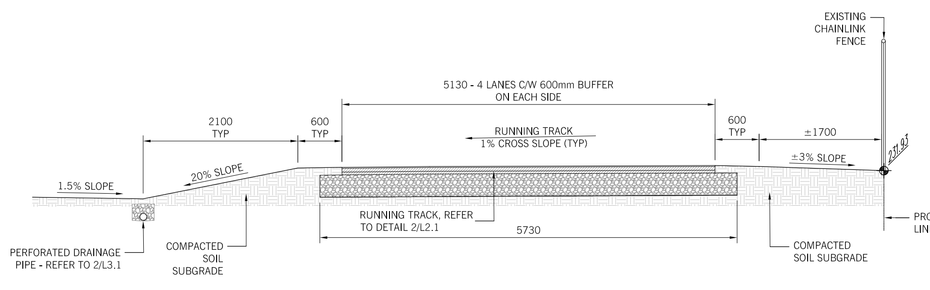
3 SECTION THROUGH TRACK - EAST SIDE L3.1 1:50
