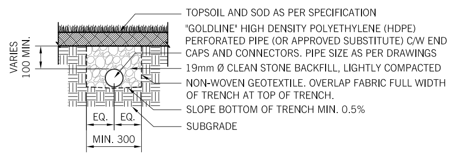
2 PERFORATED PIPE W/ FILTER CLOTH DRAINAGE SYSTEM L3.1 1:20
