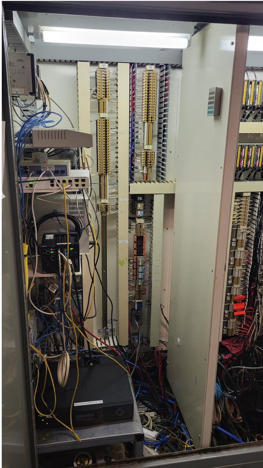
Photograph #17: Maclean Regional Pumping Station Main Control Panel Left Section
