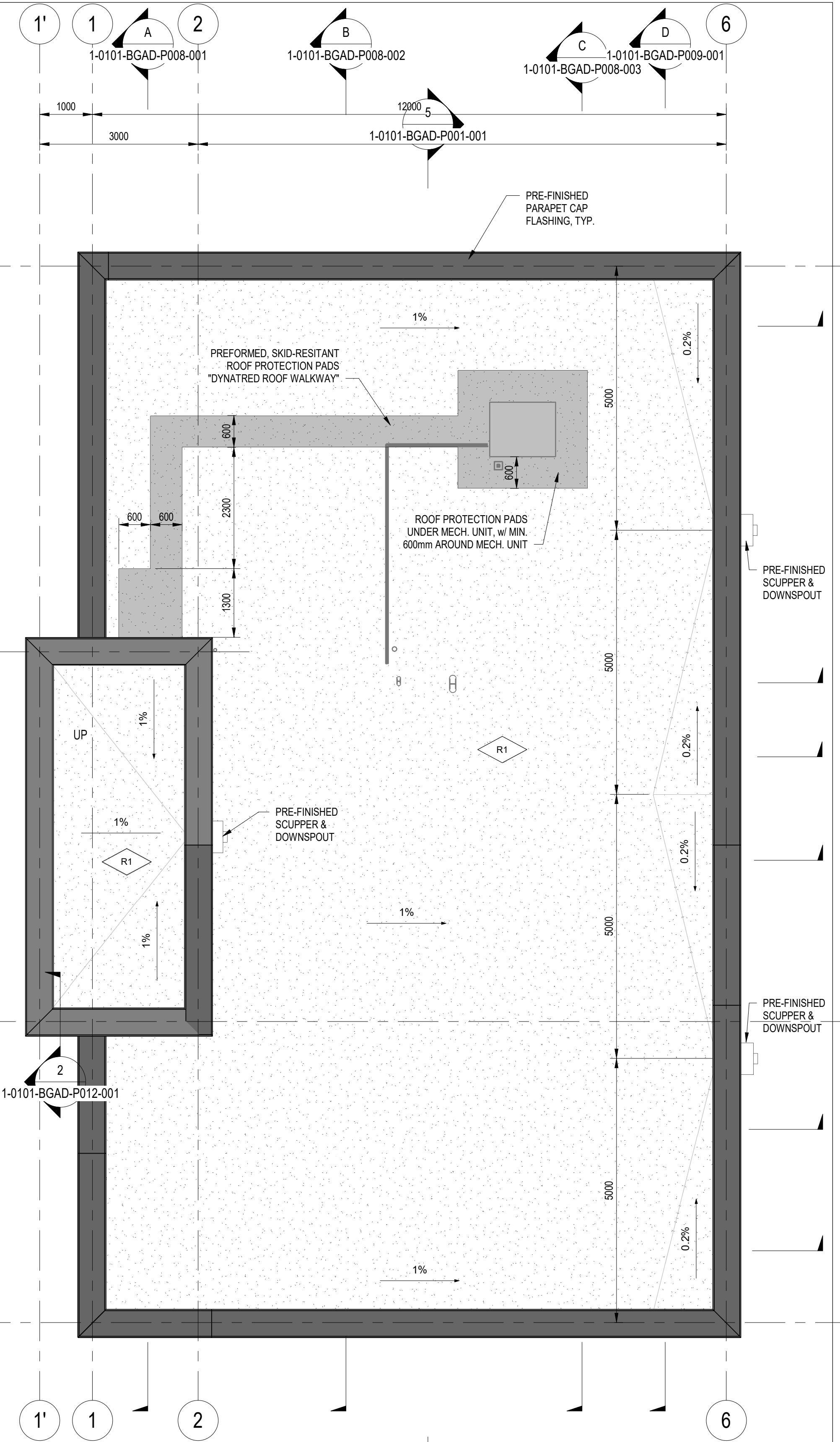
ROOF PLAN SCALE: 1 : 60
