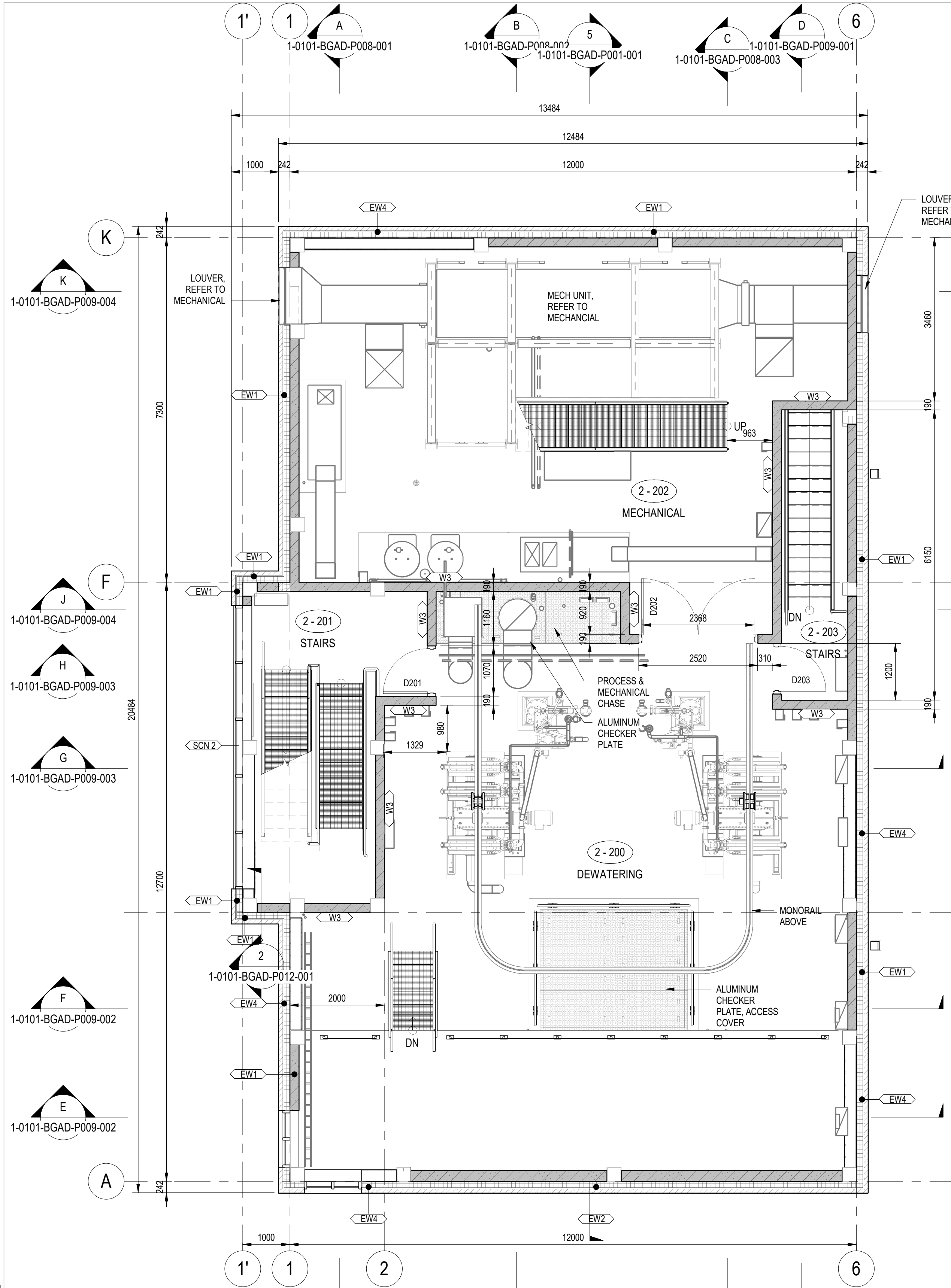
SECOND FLOOR PLAN SCALE: 1 : 60
