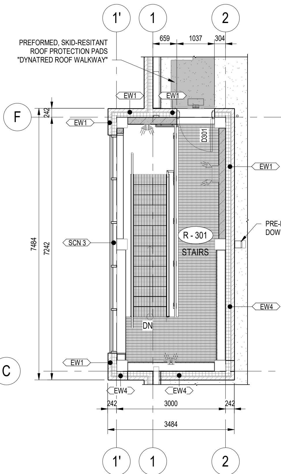
ROOF LEVEL PLAN SCALE: 1 : 60
