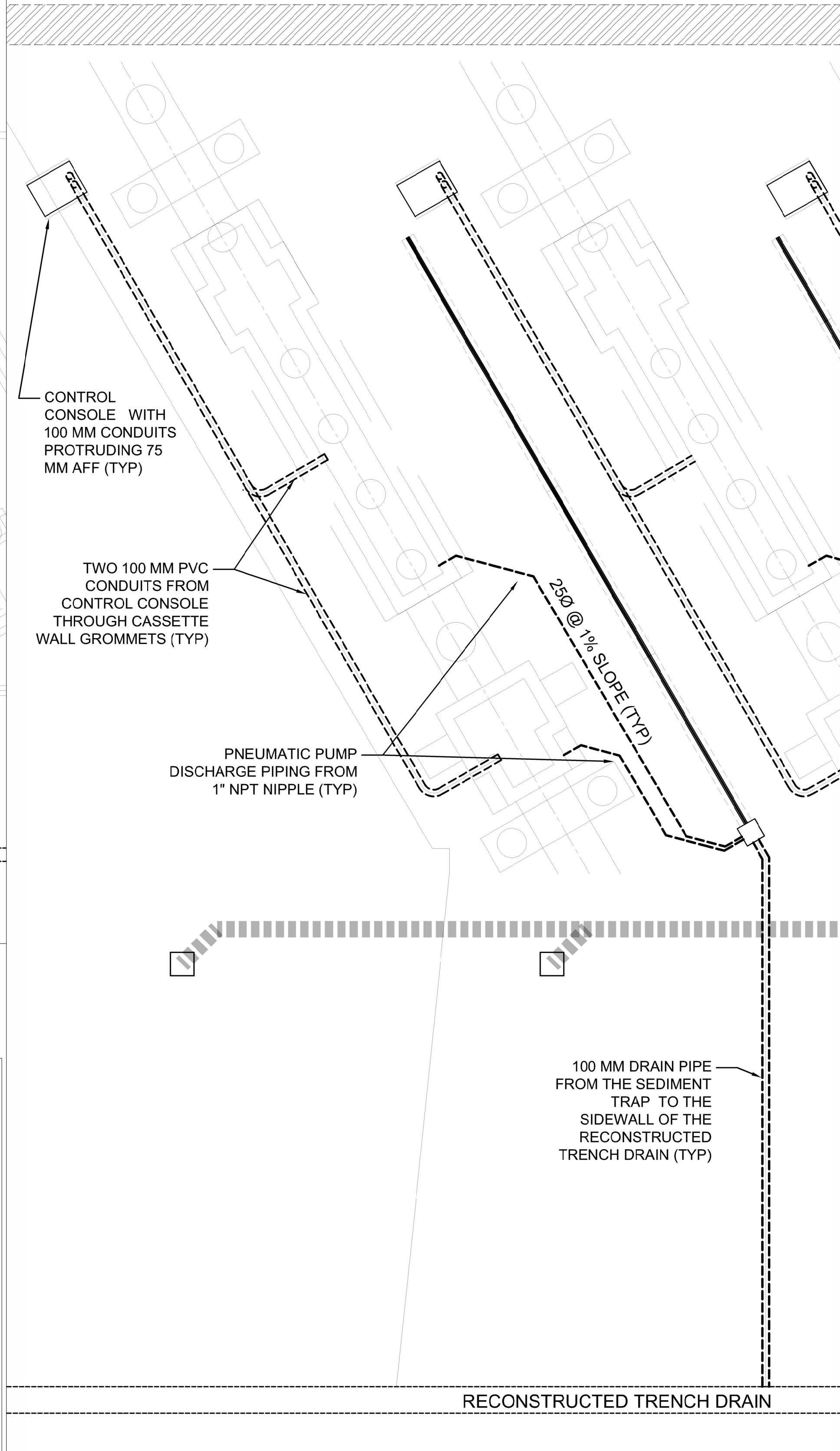
4 ENLARGED PIT INSTALLATION M-102 1:50
