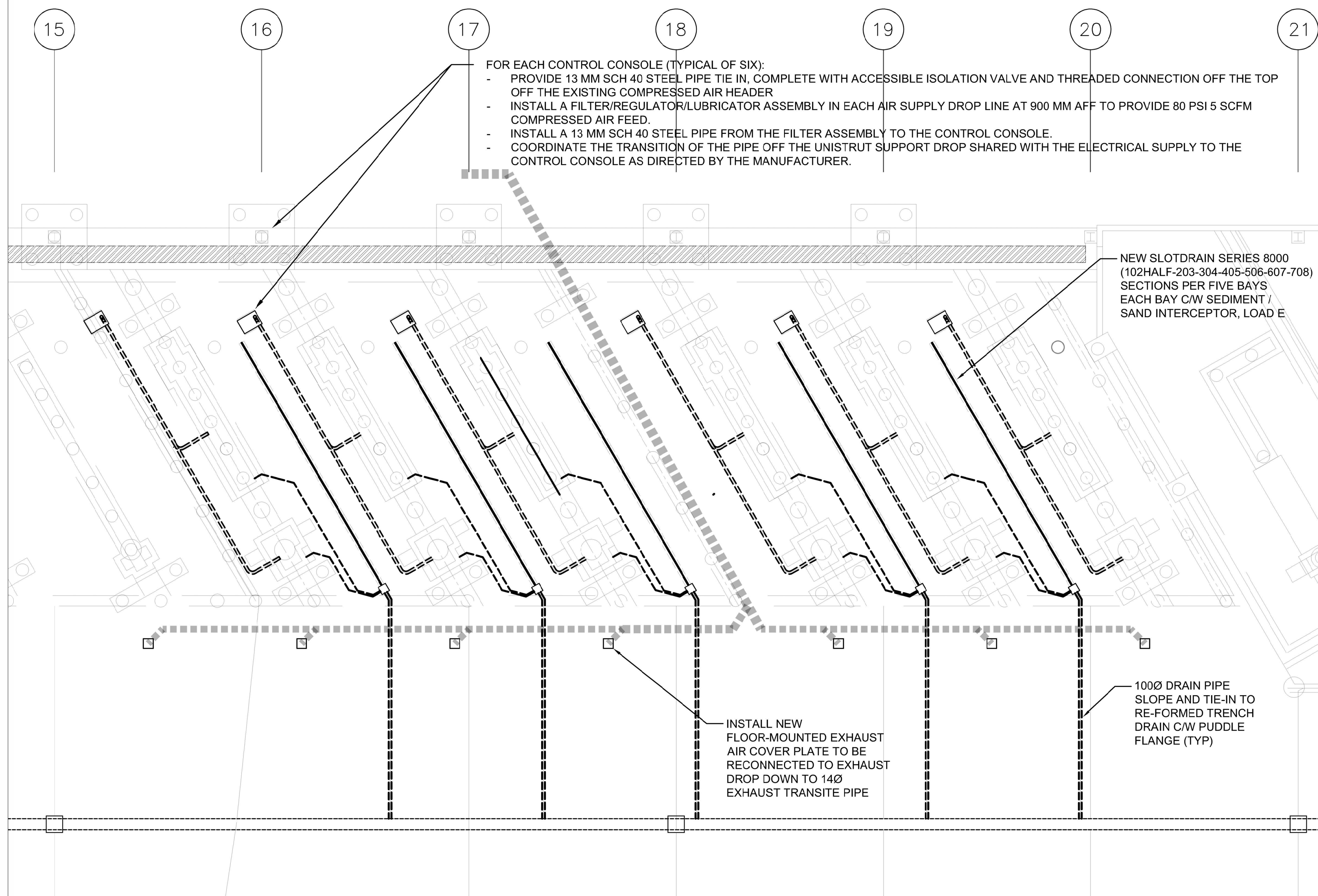
1 MAIN FLOOR PLUMBING PLAN M-102 1:100
