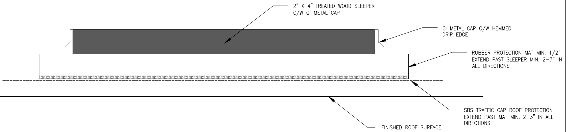
TYPICAL SLEEPER SUPPORT DETAIL
