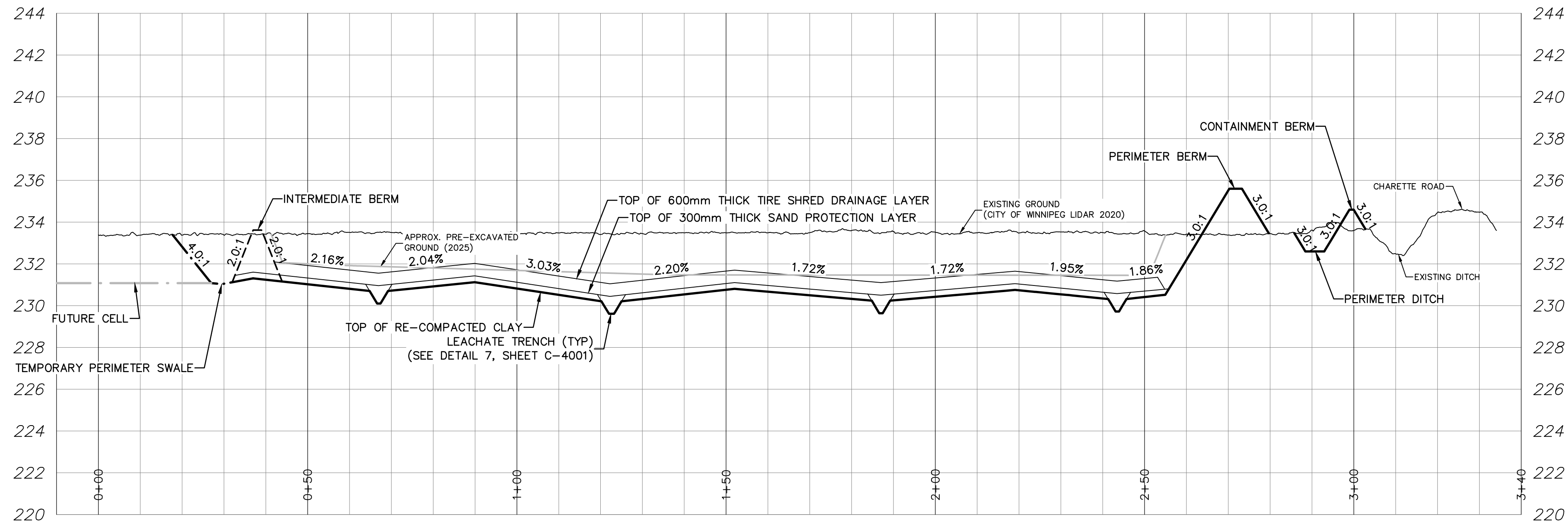
A | SECTION C-1002 Scale HORZ. 1:750 VERT. 1:100
