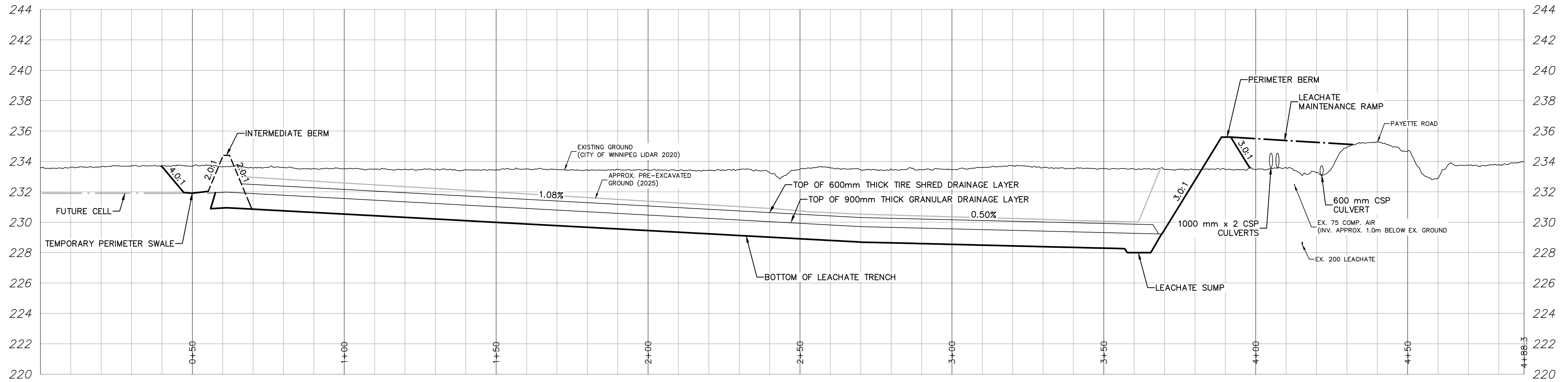
B | SECTION C-1002 Scale HORZ. 1:750 VERT. 1:100
