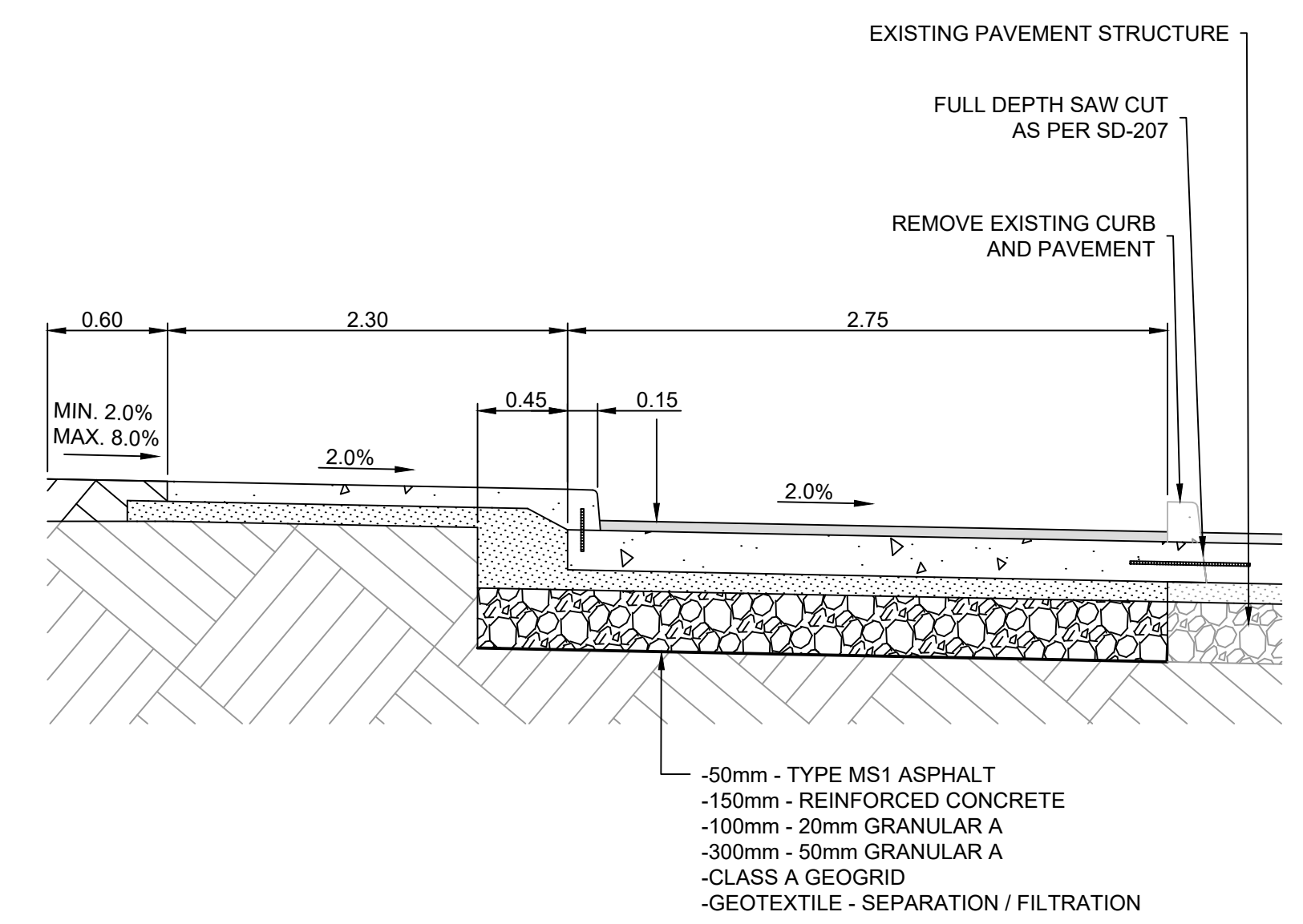
(A) DUNROBIN AVENUE PARKING LANE CROSS SECTION ('A') (SD-207, SD-228B) N.T.S.
