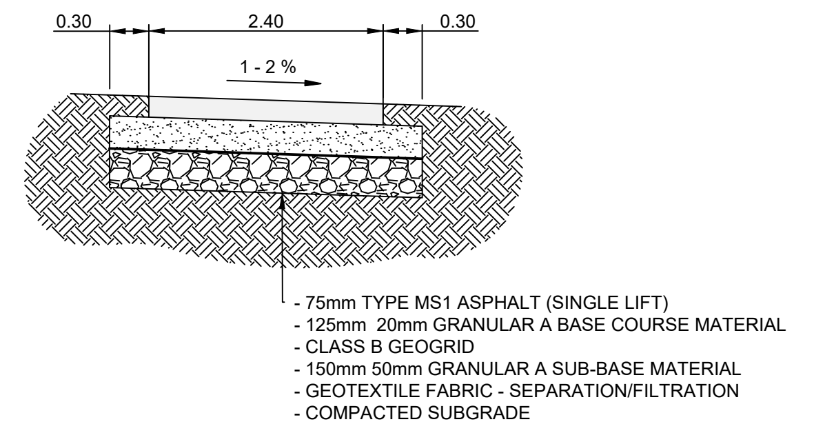
ASPHALT PAVEMENT - CROSS SECTION "A" N.T.S
