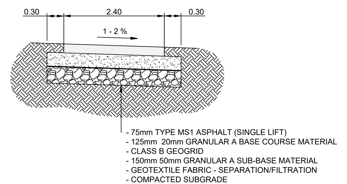
ASPHALT PAVEMENT - CROSS SECTION "A" N.T.S
