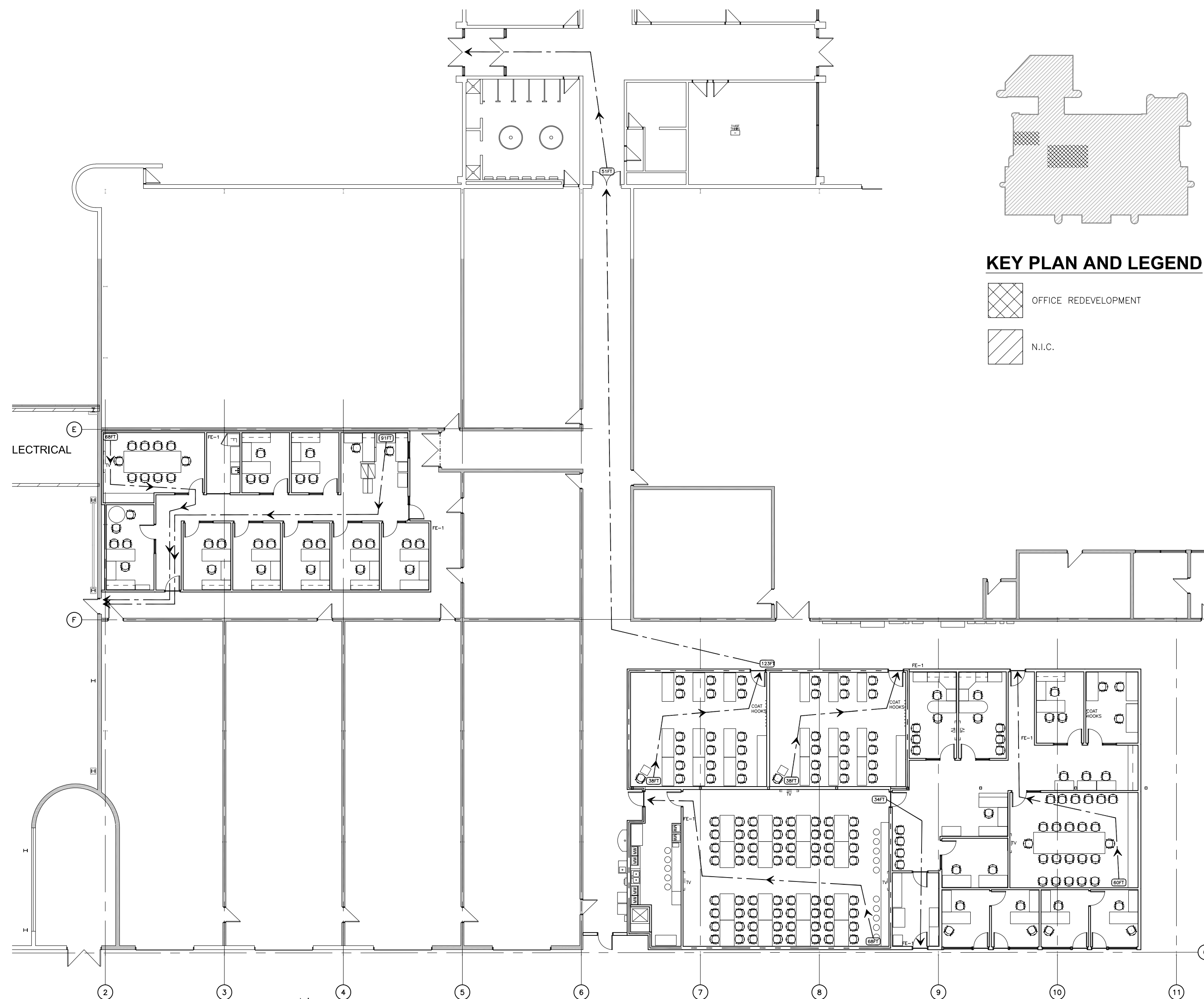
1 LIFE SAFETY PLAN AC-102 SCALE: 1/16"=1'-0"
