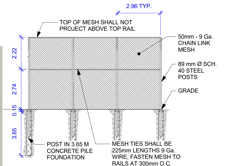
2.2 Fence Elevation Scale: 1:125
