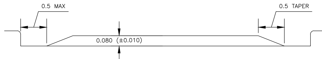
SECTION B-B
