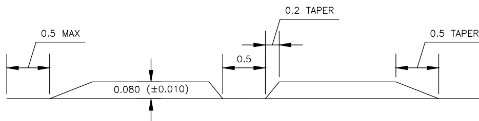
SECTION C-C
